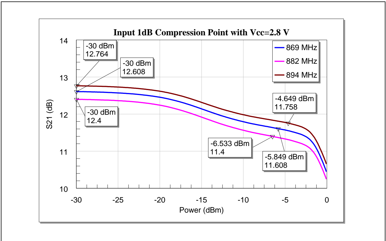
Figure 19 Input 1dB Compression Point of the BGA7L1N6 for Band-5 Applications with Vcc=2.8 V
