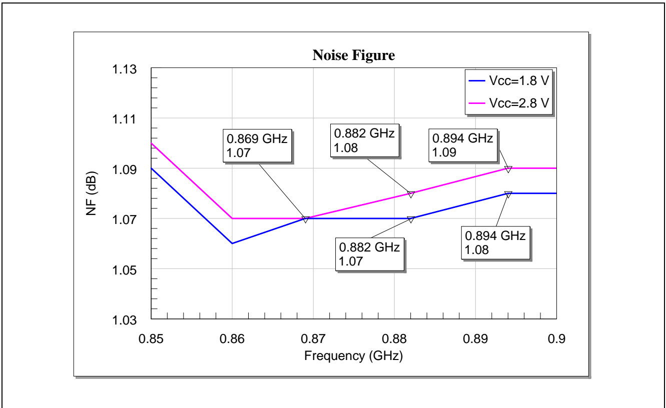
Figure 9 Noise Figure of the BGA7L1N6 for Band-5 Applications
