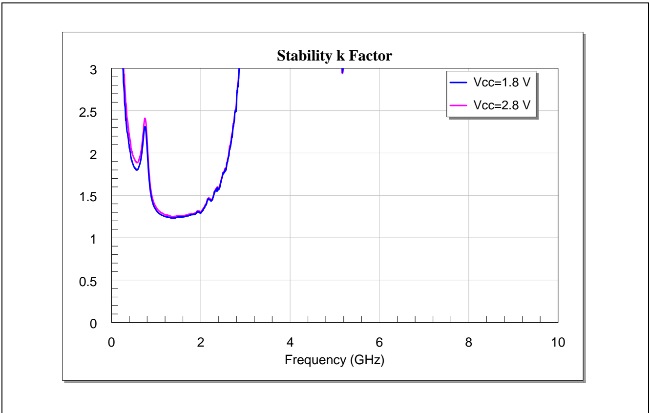
Figure 15 Stability K-factor of the BGA7L1N6 for Band-5 Applications
