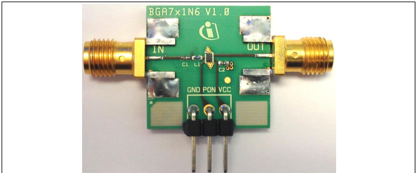
Figure 22 Picture of Evaluation Board (overview) , BGA7L1N6 V1.0
