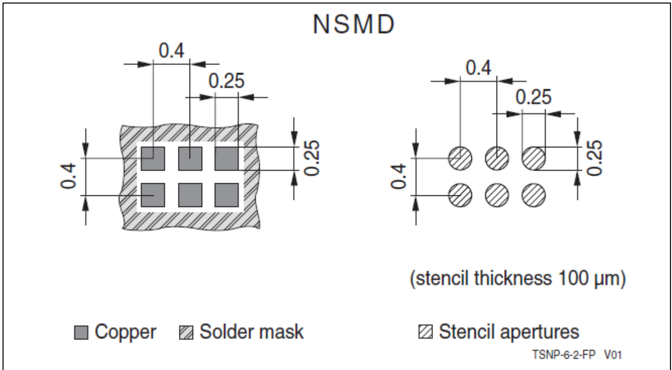
Figure 5 Footprint Recommendation of BGA7L1N6
