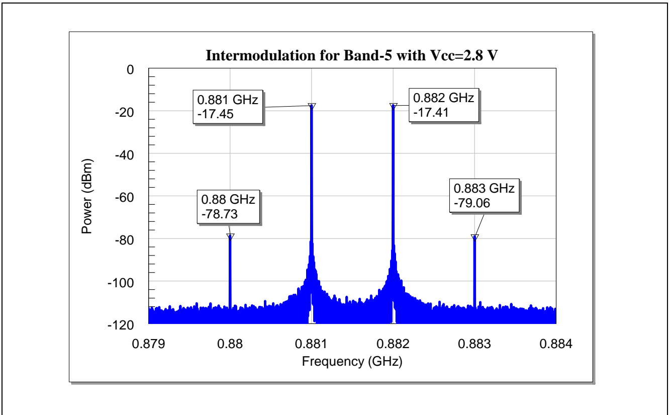
Figure 21 Input 3 rd Intercept Point of the BGA7L1N6 for Band-5 Applications with Vcc=2.8 V
