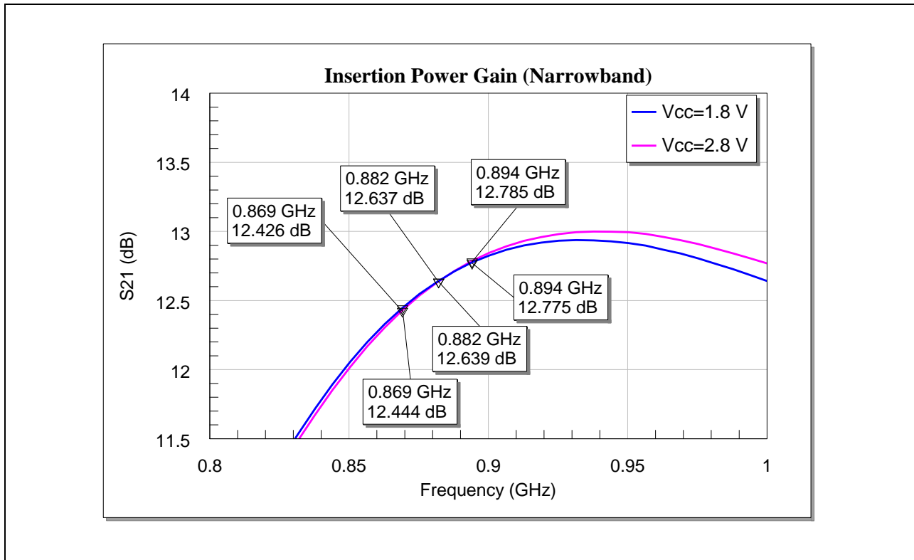
Figure 7 Insertion Power Gain (Narrowband) of the BGA7L1N6 for Band-5 Applications
