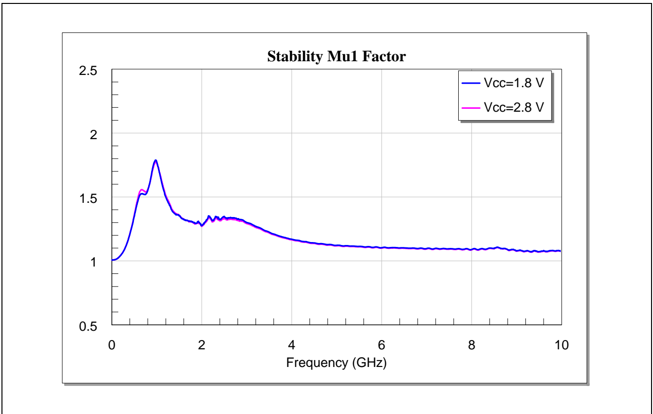
Figure 16 Stability Mu1-factor of the BGA7L1N6 for Band-5 Applications
