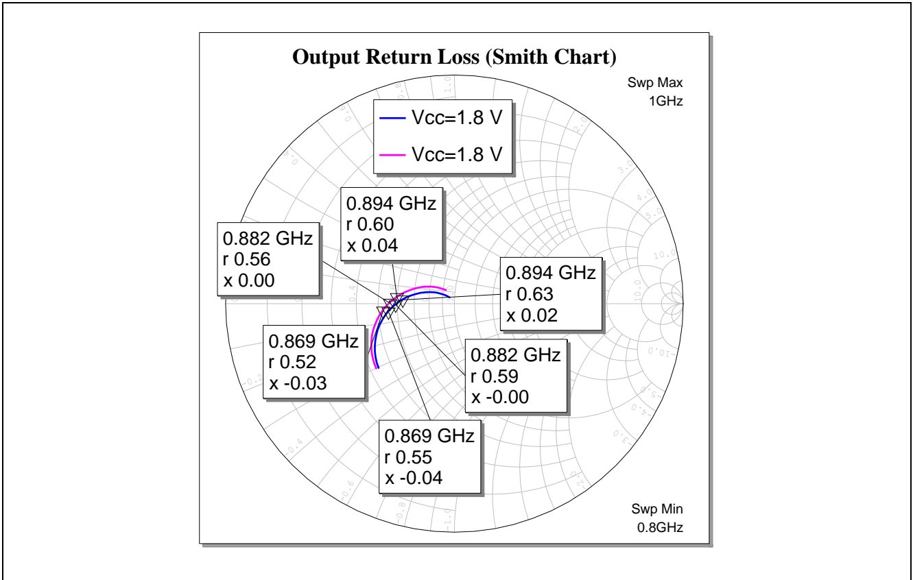
Figure 13 Output Matching (Smith Chart) of the BGA7L1N6 for Band-5 Applications
