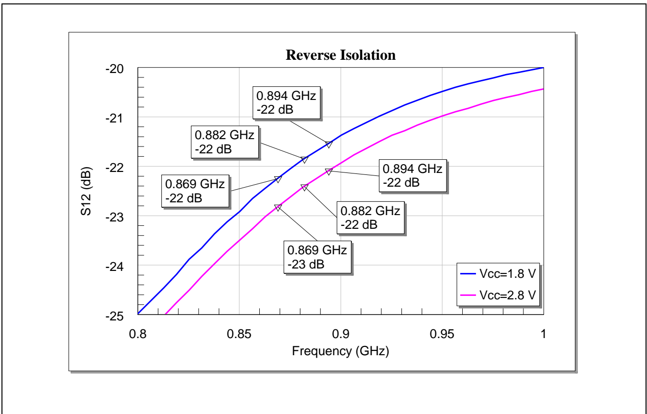
Figure 14 Reverse Isolation of the BGA7L1N6 for Band-5 Applications
