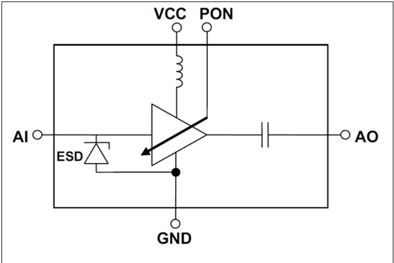
Figure 3 Equivalent Circuit of BGA7L1N6
