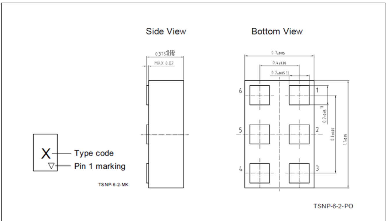
Figure 4 Package and Pin Connections of BGA7L1N6
