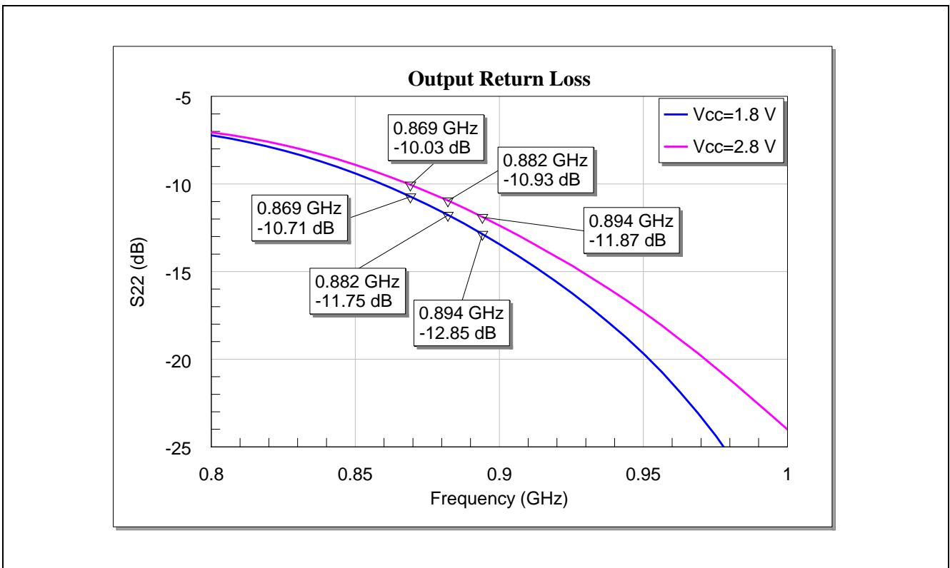
Figure 12 Output Matching of the BGA7L1N6 for Band-5 Applications
