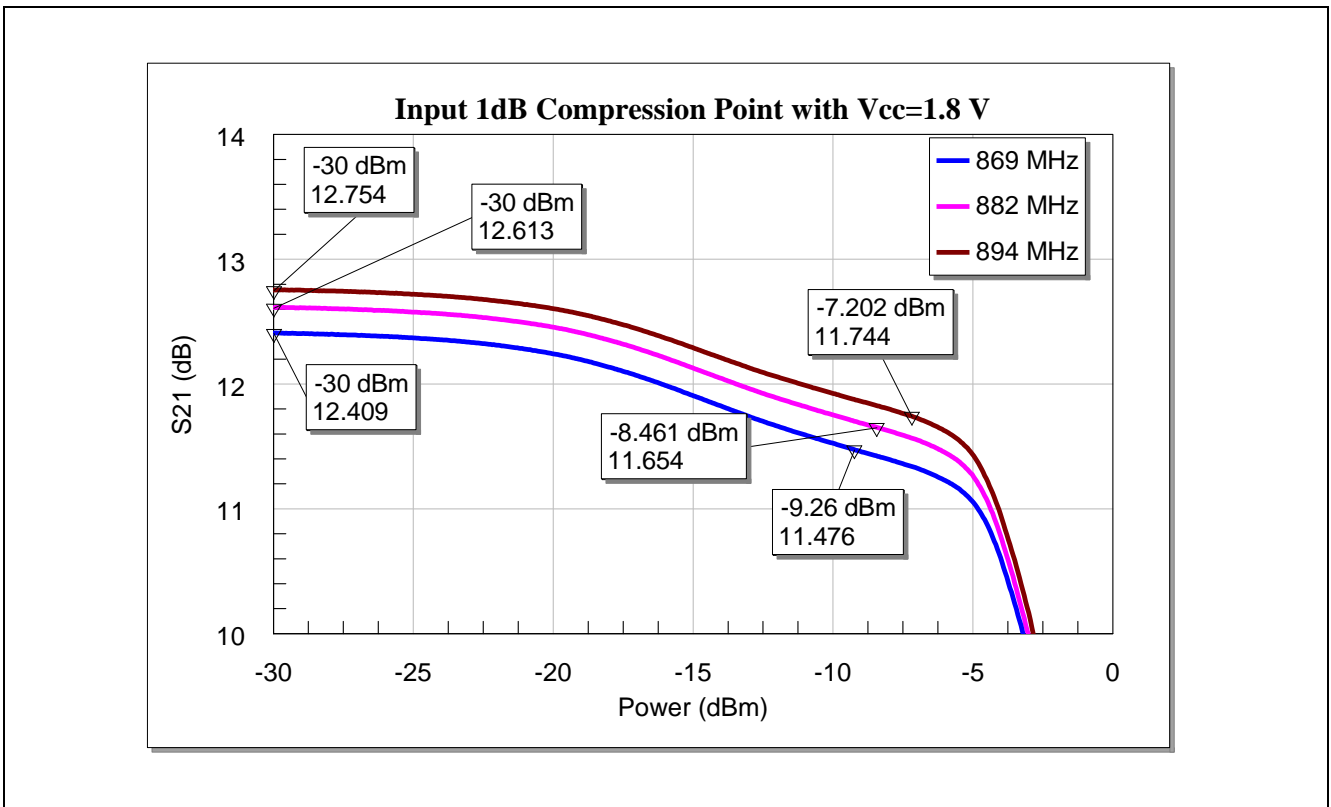
Figure 18 Input 1dB Compression Point of the BGA7L1N6 for Band-5 Applications with Vcc=1.8 V
