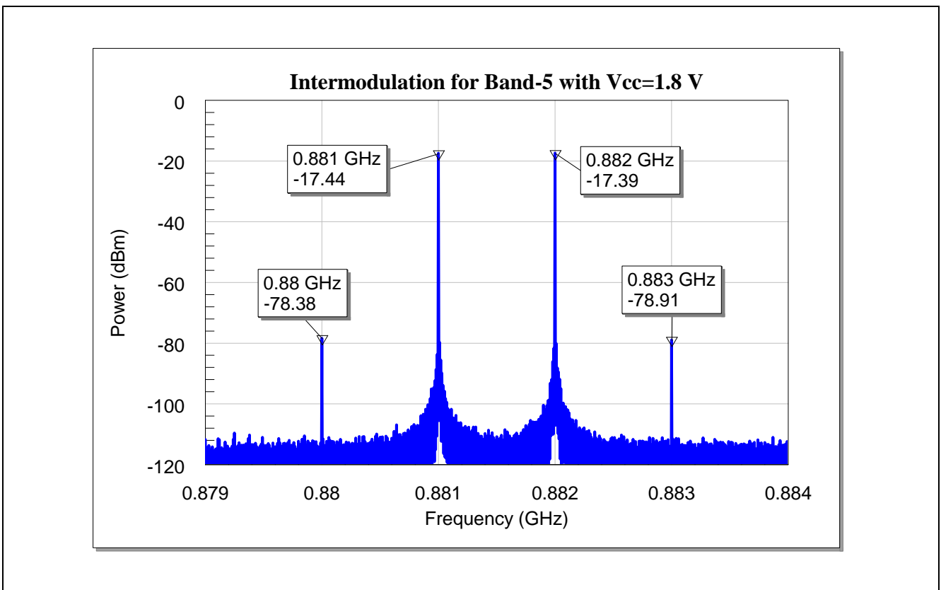
Figure 20 Input 3 rd Intercept Point of the BGA7L1N6 for Band-5 Applications with Vcc=1.8 V
