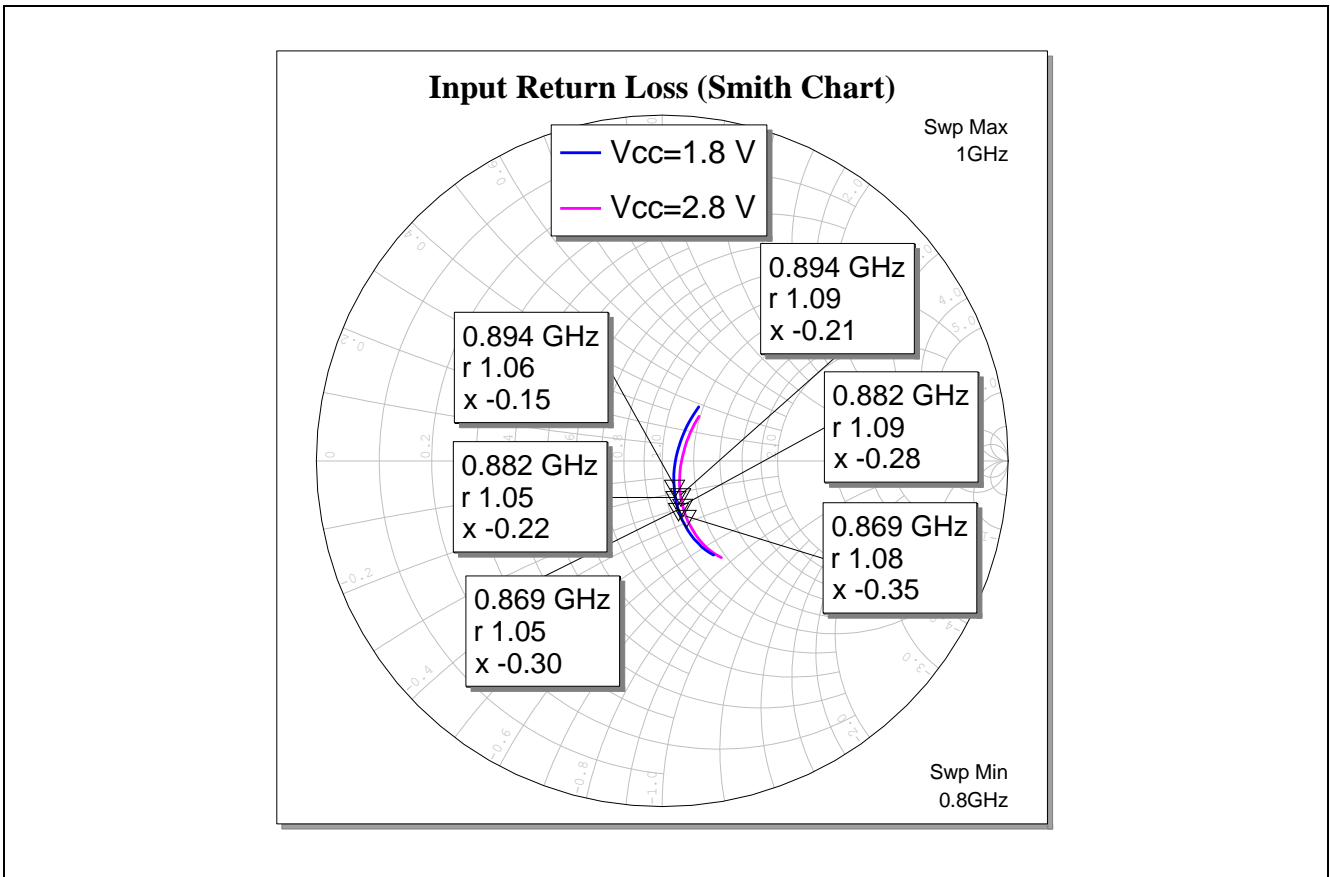
Figure 11 Input Matching (Smith Chart) of the BGA7L1N6 for Band-5 Applications
