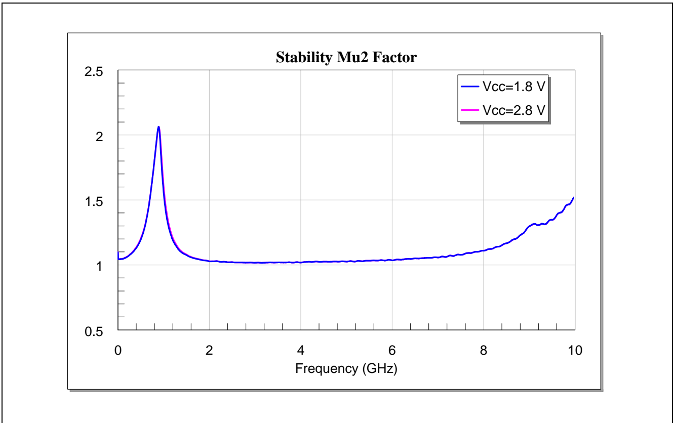
Figure 17 Stability Mu2-factor of the BGA7L1N6 for Band-5 Applications
