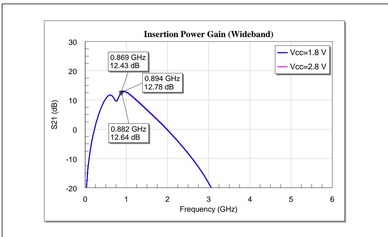
Figure 8 Insertion Power Gain (Wideband) of the BGA7L1N6 for Band-5 Applications
