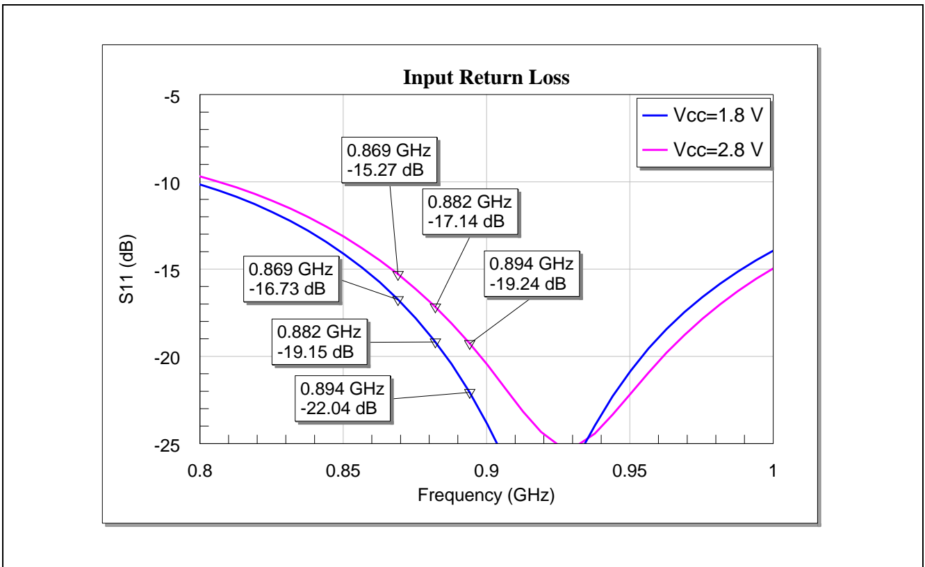
Figure 10 Input Matching of the BGA7L1N6 for Band-5 Applications
