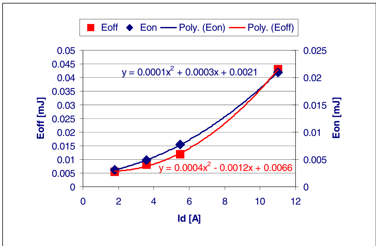
Figure 5 Switching Energy Losses vs. Drain Current (SPP11N60C3, SDP06S60, R_{gate} = 6.8 \Omega , V_{ds} = 380 \text{ V} , T_J = 125^\circ\text{C} )
