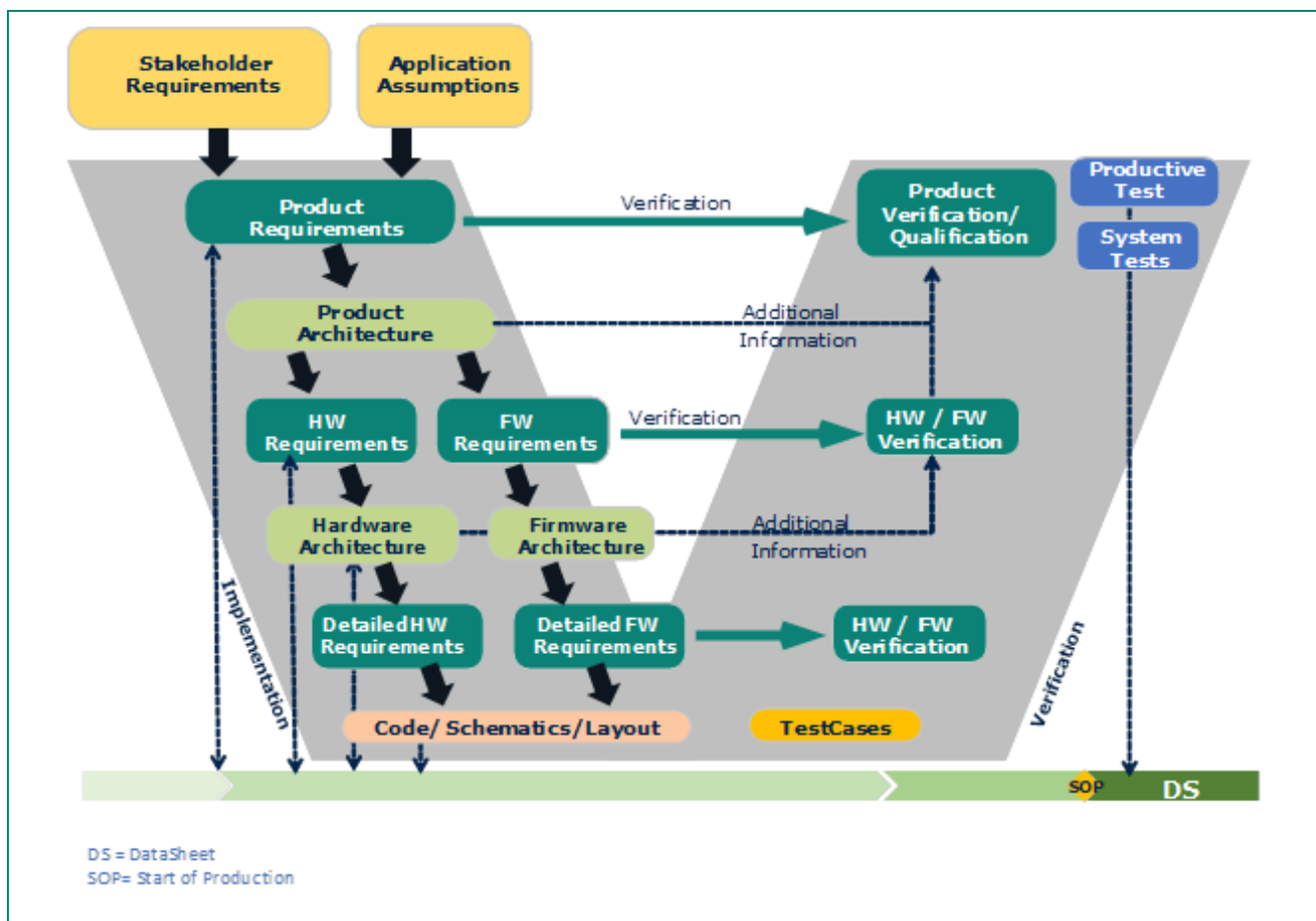
Figure 1 Requirements Based development in accordance with ISO 26262 (Source: Infineon)
