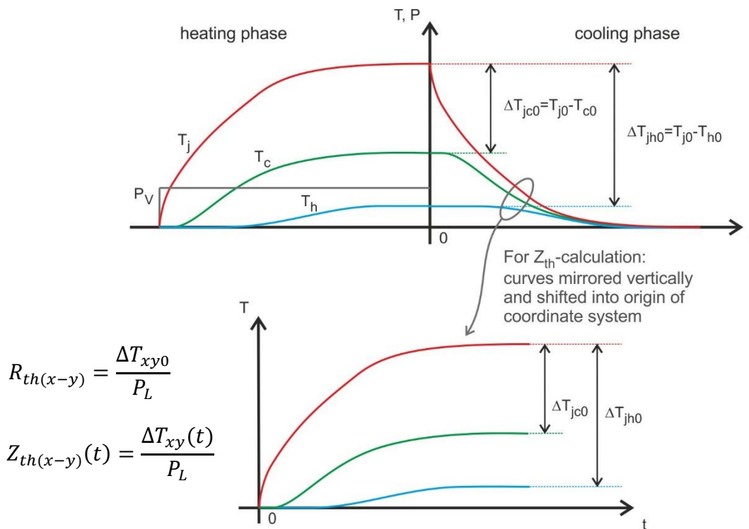
Figure 1 Principle approach of thermal impedance measurement
