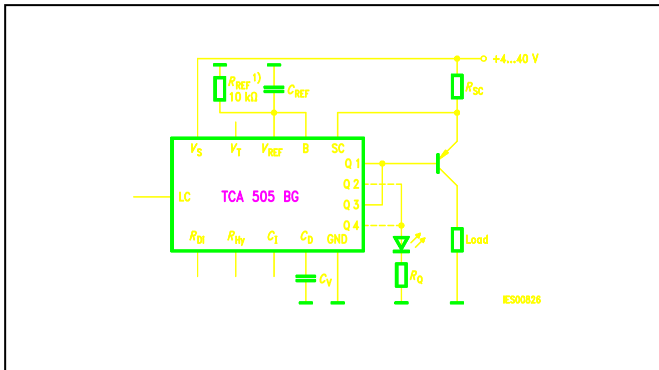
Application Circuit 2
