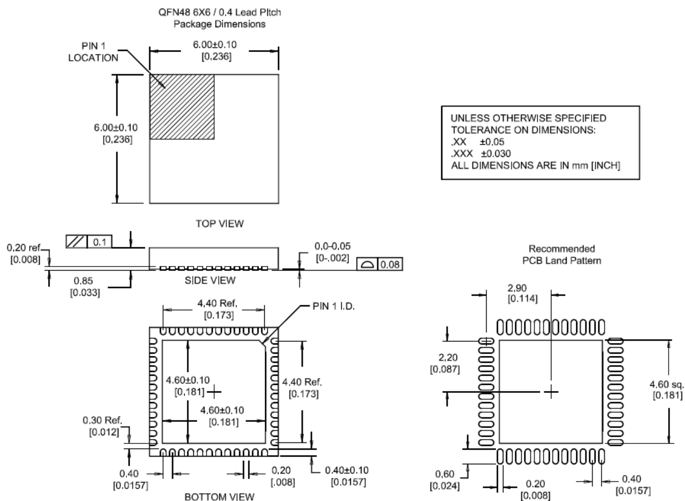
Figure 4: Package Dimensions
