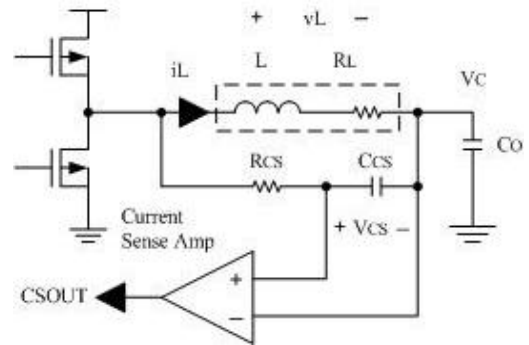
Figure 9: Inductor Current Sensing and Current Sense Amplifier
