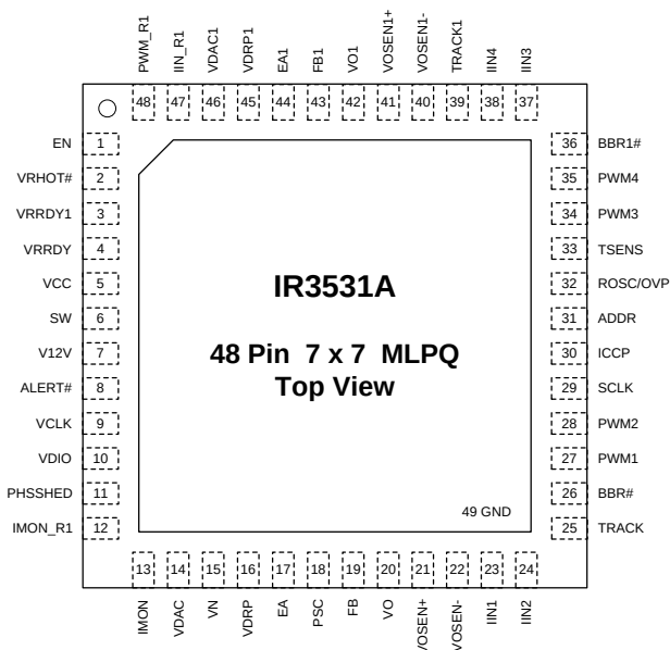
Figure 2: IR3531A Package Top View
