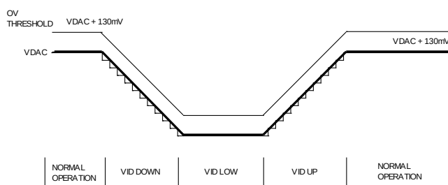
Figure 16: Over Voltage Protection during SETVID Fast/Slow
