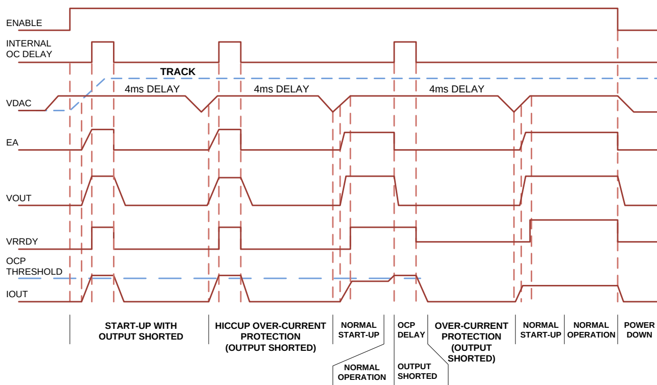
Figure 14: Over-Current Waveforms during and after start-up
