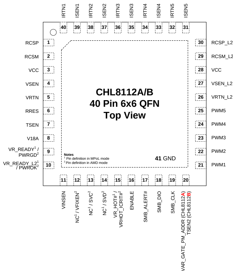
Figure 1. CHL8112A & CHL8112B Packages
