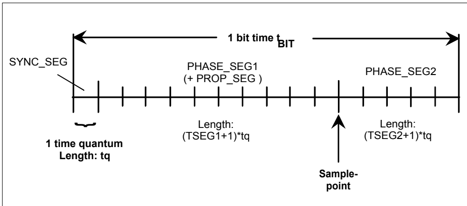
Figure 17 Rough Structure of one Bit Cell in the CAN Module of the C167CR / C515C and in the SAE 81C90/91
