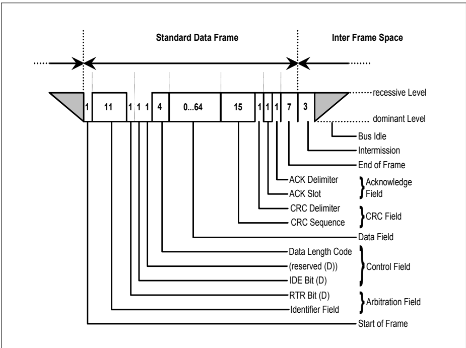
Figure 1 Standard CAN Data Frame
