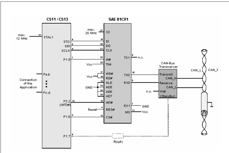
Figure 16 Connection of a C511 / C513 to CAN via the SAE 81C91 (serial)
