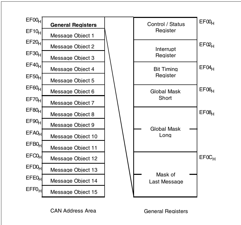
Figure 9 CAN addressing area on the C167CR
