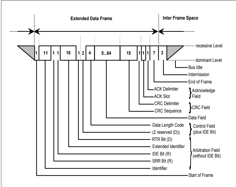
Figure 2 Extended CAN Data Frame
