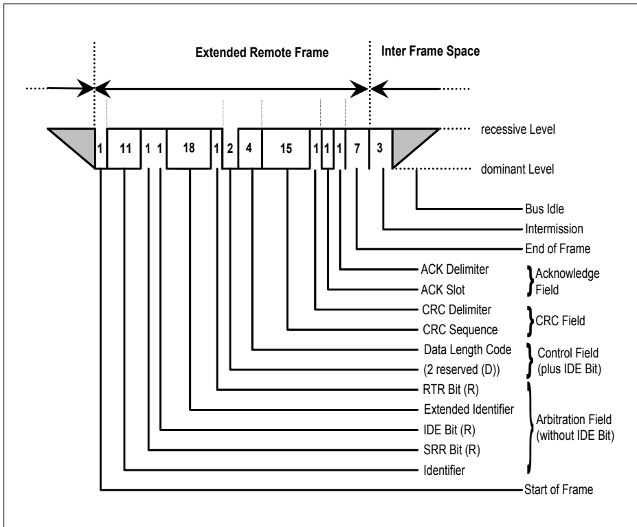
Figure 4 Extended CAN Remote Frame
