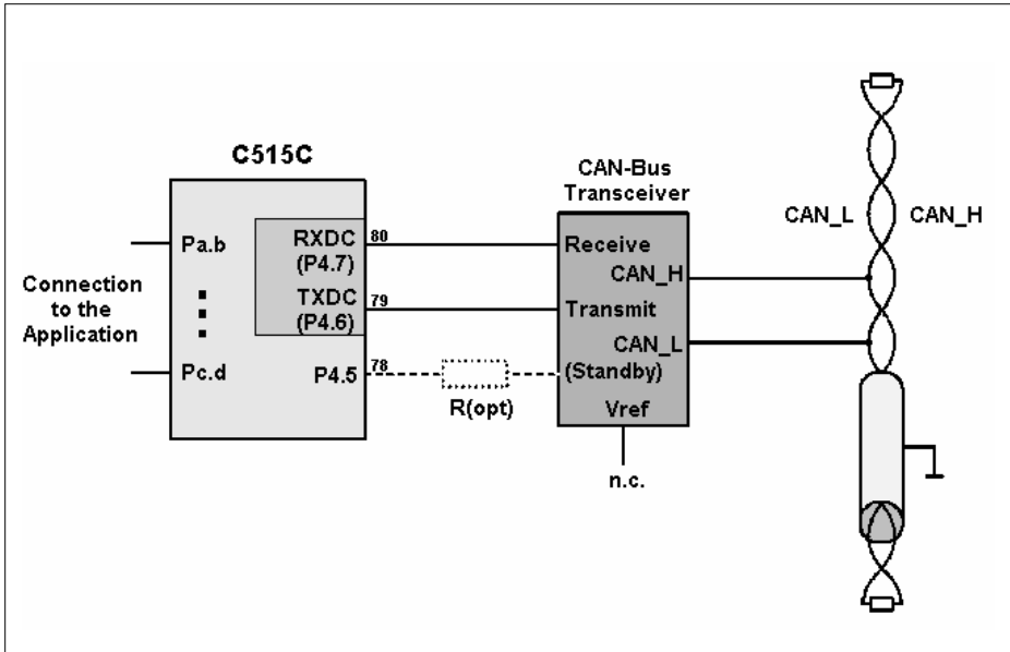
Figure 14 Connection of a C515C to CAN
