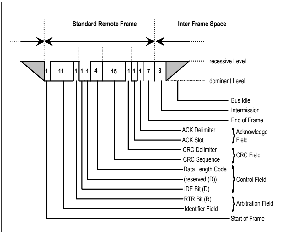
Figure 3 Standard CAN Remote Frame
