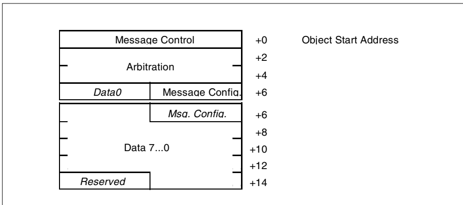
Figure 11 Message Objects in the C167CR
