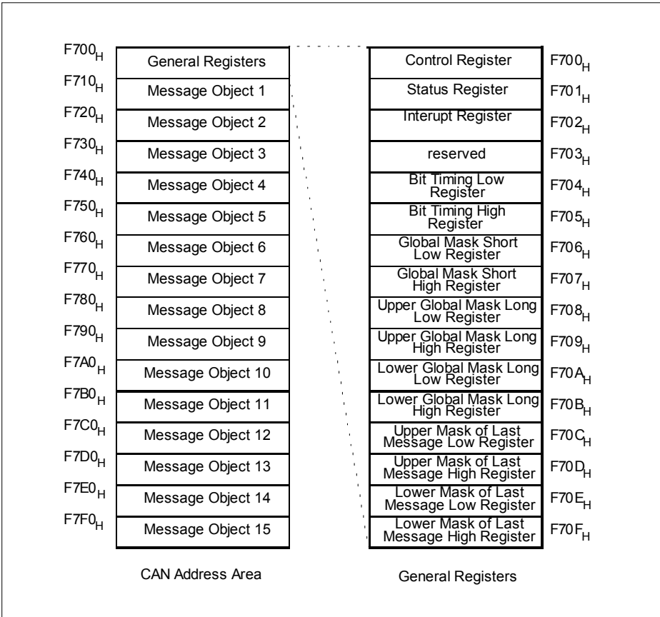
Figure 8 CAN addressing area on the C515C
