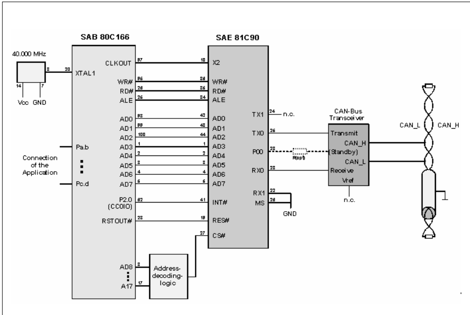
Figure 15 Connection of a SAB 80C166 to CAN via the SAE 81C90 (parallel)
