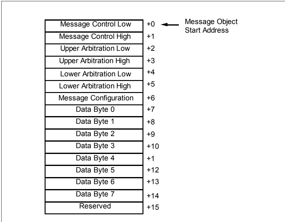
Figure 10 Message Objects in the C515C
