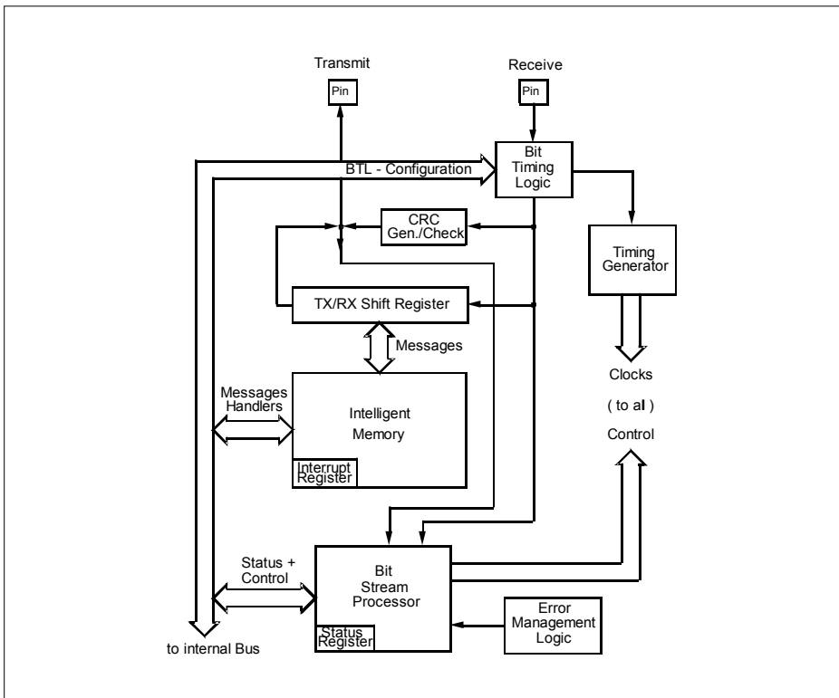
Figure 7 Block Diagram of the CAN Controller on the C167CR / C515C
