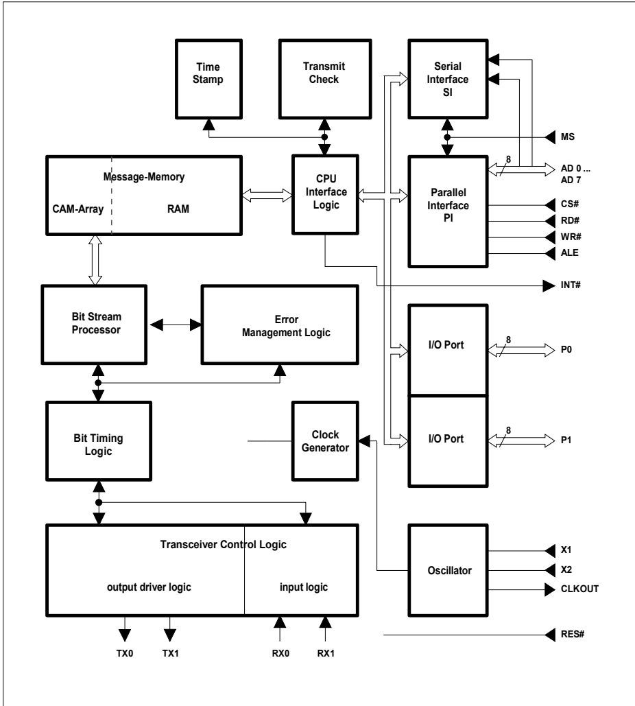
Figure 12 Block Diagram of the SAE 81C90/91 (I/O Ports only available for SAE 81C90)
