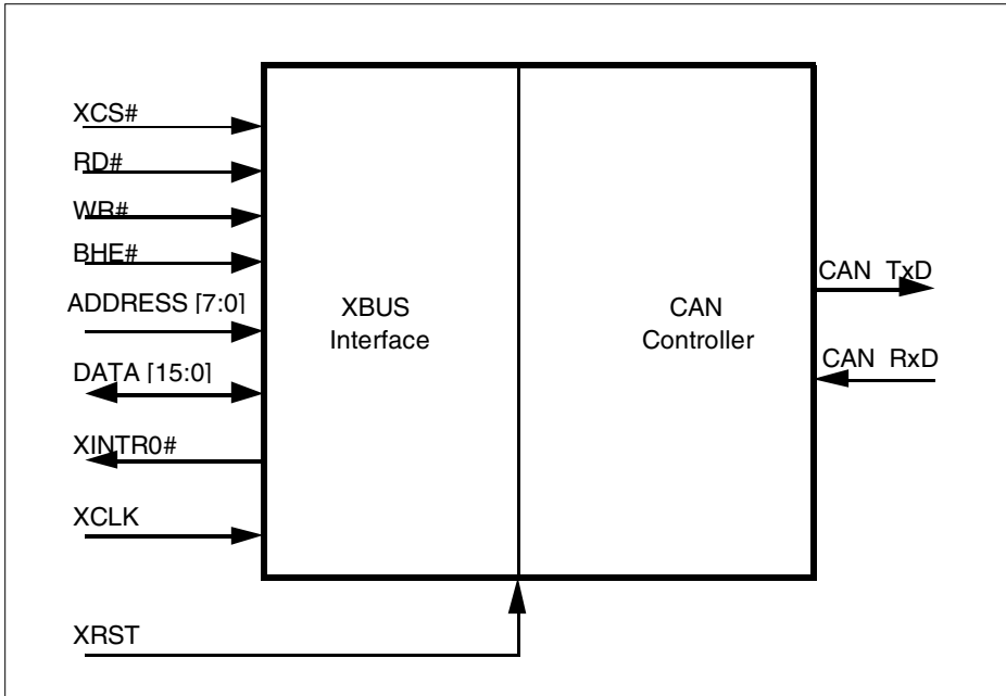
Figure 6 Block Diagram of the CAN module (connected to the C167CR here)
