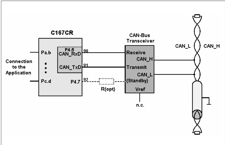
Figure 13 Connection of the C167CR to CAN
