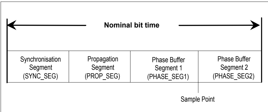
Figure 5 Partition of bit time
