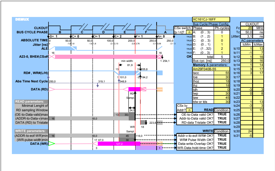
Figure 11 Sheet Layout for Timing Calculations in DEMUX Mode.
