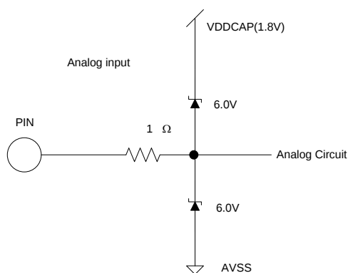
Figure 22. Analog input
