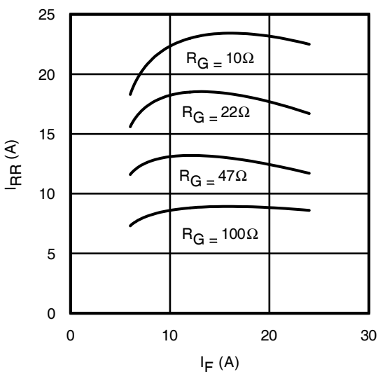
Fig. 17 - Typ. Diode I_{\text{RR}} vs. I_F
