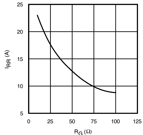
Fig. 18 - Typ. Diode I_{\text{RR}} vs. R_G
