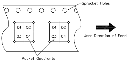
QUADRANT ASSIGNMENTS FOR PIN 1 ORIENTATION IN TAPE
