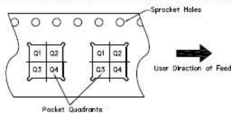
QUADRANT ASSIGNMENTS FOR PIN 1 ORIENTATION IN TAPE
