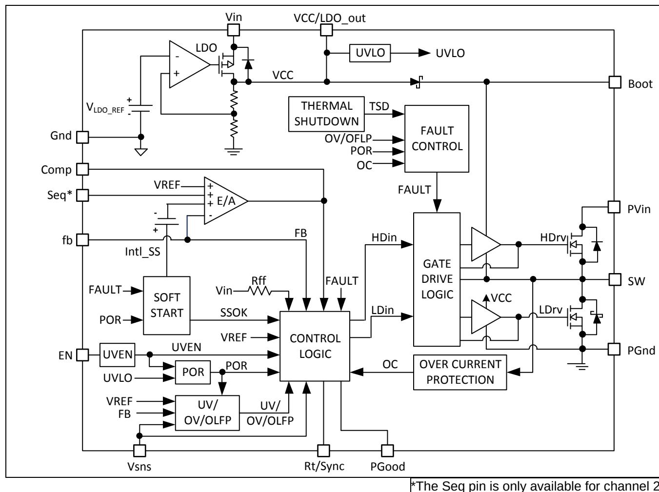
Figure 3: IR3892 Simplified Block Diagram (one phase)
