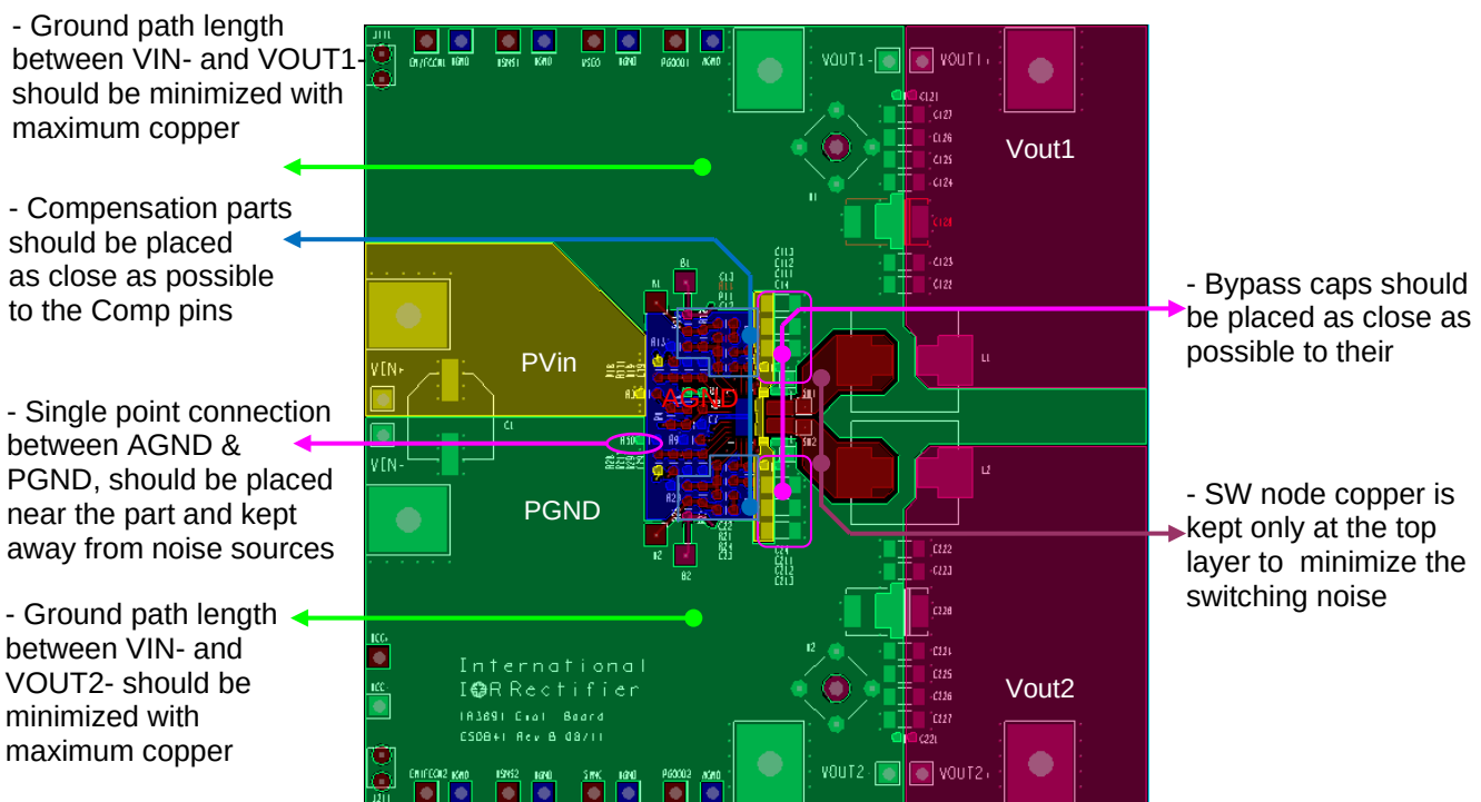
Figure 42a: IRDC3891 Demo board Layout Considerations – Top Layer
