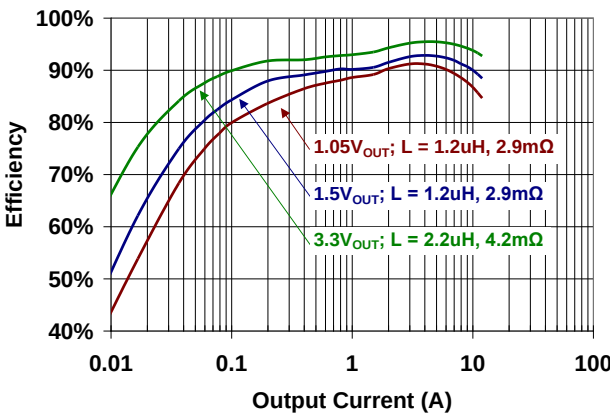
Figure 2. Efficiency vs. Output Current for V_{IN} = 12.6V
