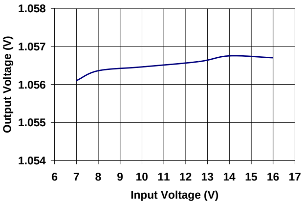
Figure 6. Output Voltage Regulation vs. Input Voltage at I_{OUT} = 12A
