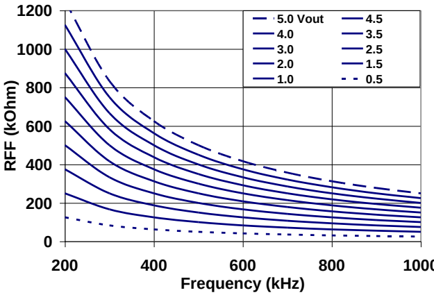
Figure 4. Frequency vs. R_{FF}
