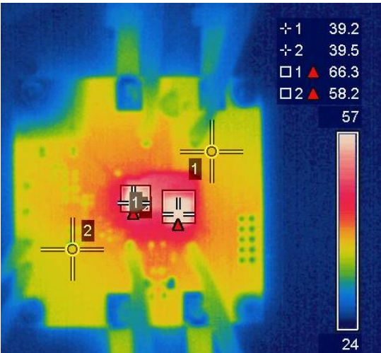
Figure 16: Thermal Image at VIN = 12V, IOUT = 8A (IR3871: 66°C, Inductor: 58°C, PCB: 40°C)
