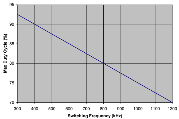
Fig. 10. Maximum duty cycle v/s switching frequency.
