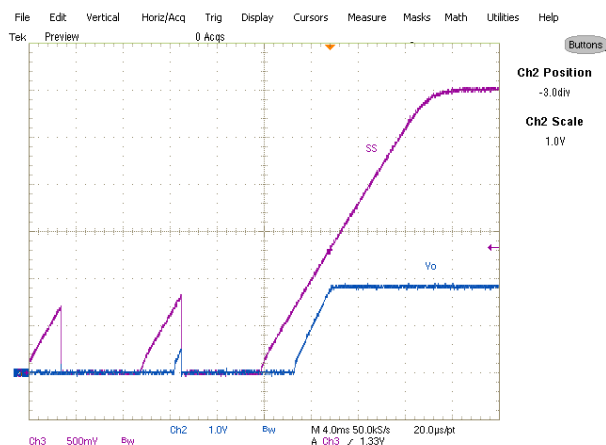
Fig. 22. Short (Hiccup) Recovery Ch 2 :V 0 , Ch 3 :V SS
