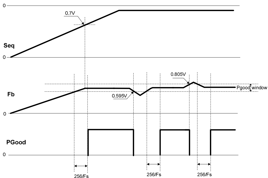
Fig.9b IR3843W Tracking Operation
