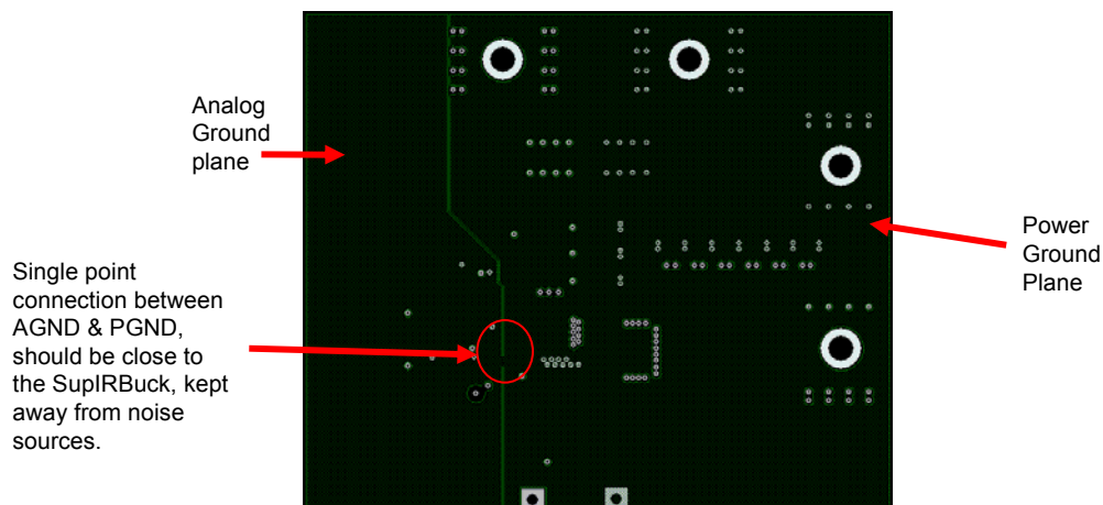
Fig. 26c. IRDC3843A demoboard layout considerations – Mid Layer 1
