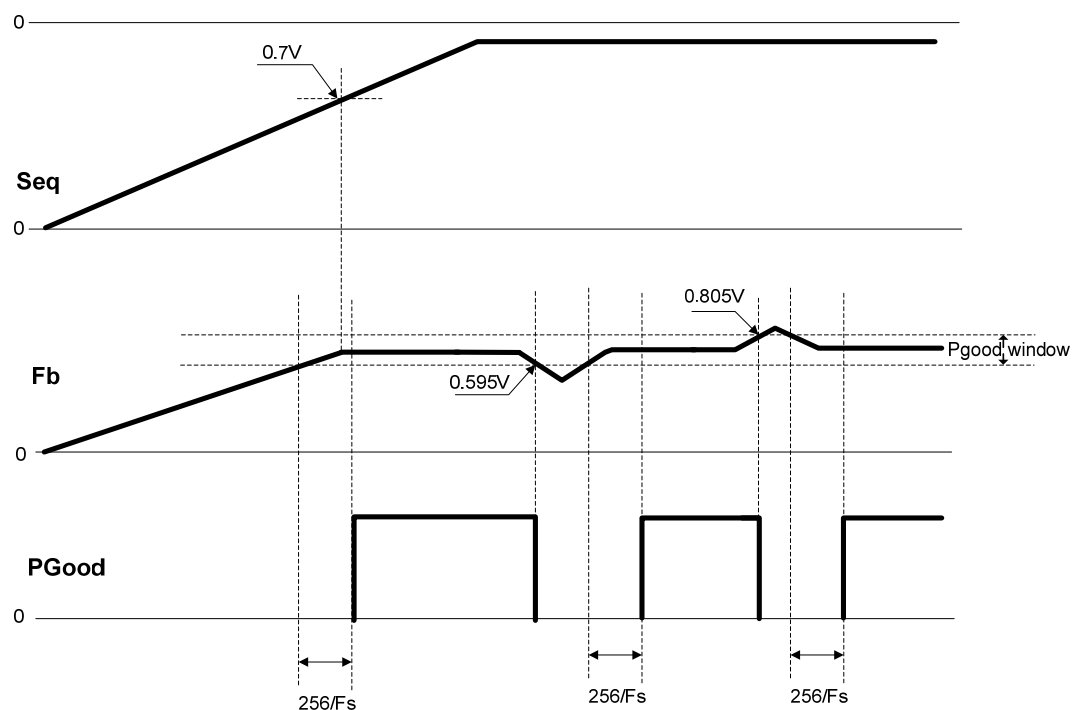
Fig.9b IR3843A Tracking Operation
