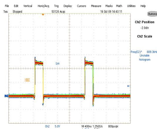
Fig. 21: Inductor node at 12A load Ch 2 :LX
