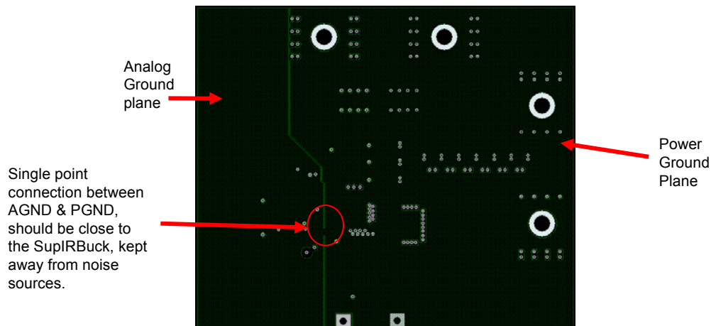
Fig. 26c. IR3832W layout considerations – Mid Layer 1
