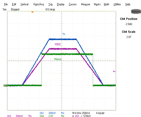
Fig. 22: Tracking 4A, sourcing current, Ch_2:V_{out} , Ch_3:V_{DDQ} , Ch_4:PGood
