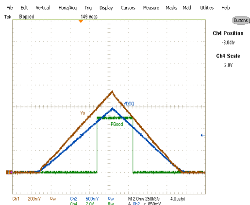
Fig. 22: Tracking 8A, sourcing current, Ch_1:V_{out} , Ch_3:V_{DDQ} , Ch_4:PGood
