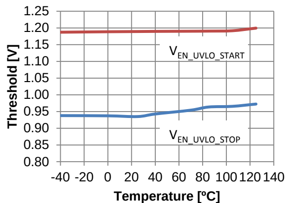
Figure 17: EN Threshold vs. Temperature
