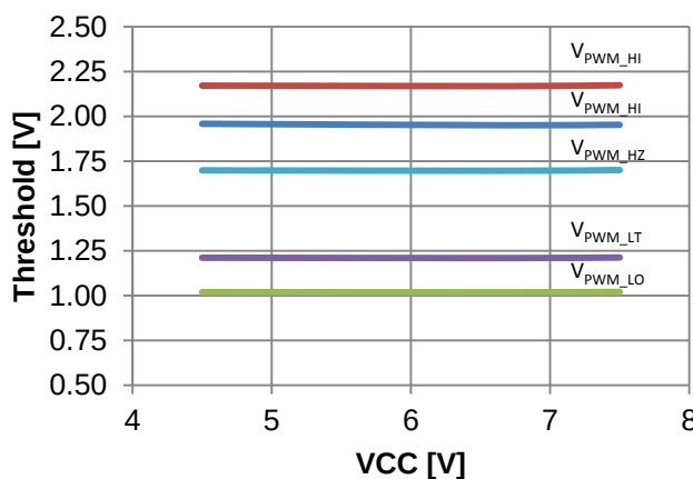
Figure 14: PWM Threshold vs. Driver Supply Voltage
