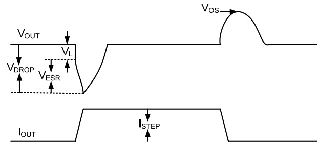
Figure 23. Typical Output Voltage Response Vaveform.
