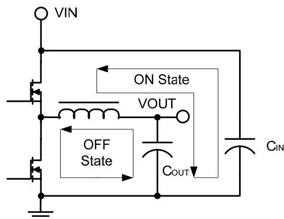
Figure 24. Current Path of Power Stage
