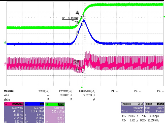
Figure 15. Input Voltage Step at 2A Load with 0.1V/uS
