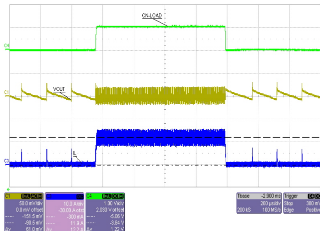
Figure 13. Load Step Transient in CCM @ Vin = 19V
