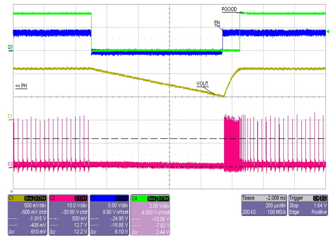
Figure 16. Over Current Protection at 30A
