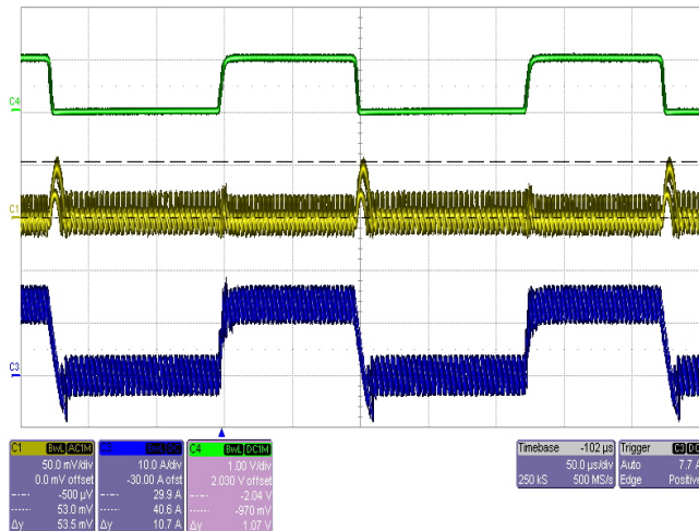
Figure 12. Frequency Variation less than 10% at 20A Load
