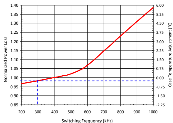
Figure 12: Normalized Power Loss vs. Switching Frequency
