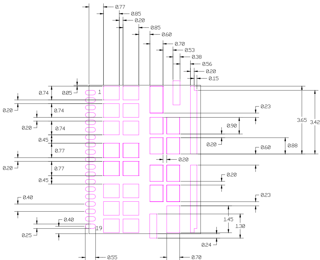
Figure 36: Stencil design
