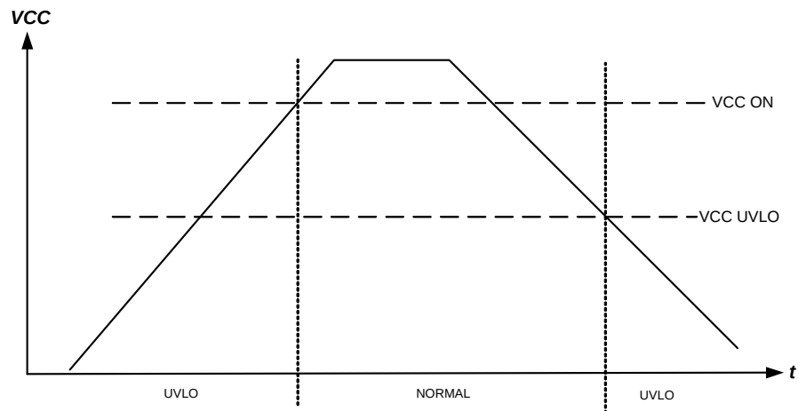
Figure 5: Vcc UVLO
