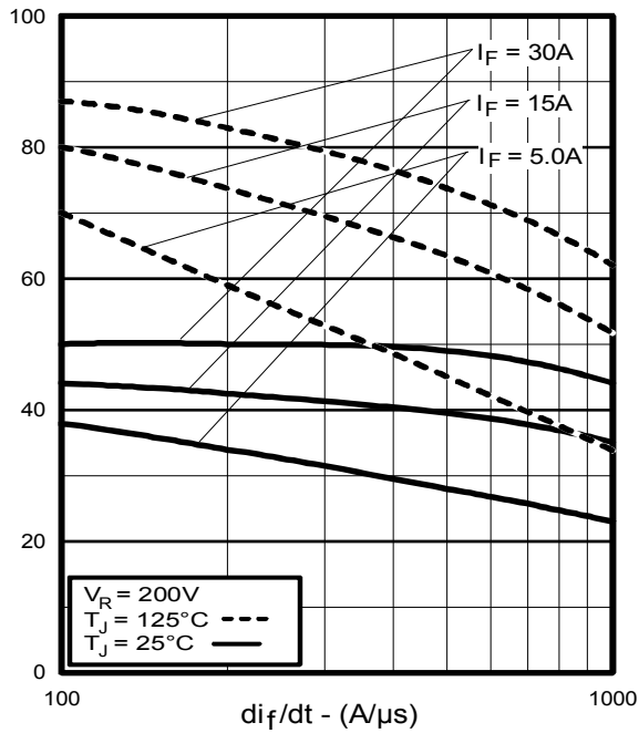
Fig. 5 - Typical Reverse Recovery vs. di/dt
