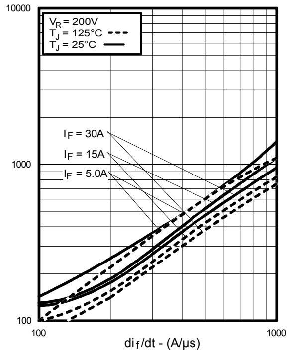
Fig. 8 - Typical di_{(rec)}M/dt vs. di/dt
