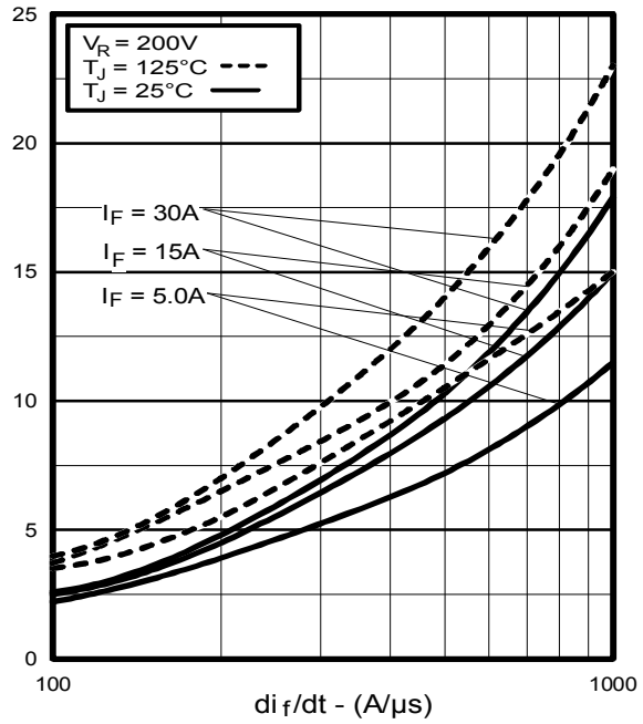
Fig. 6 - Typical Recovery Current vs. di/dt
