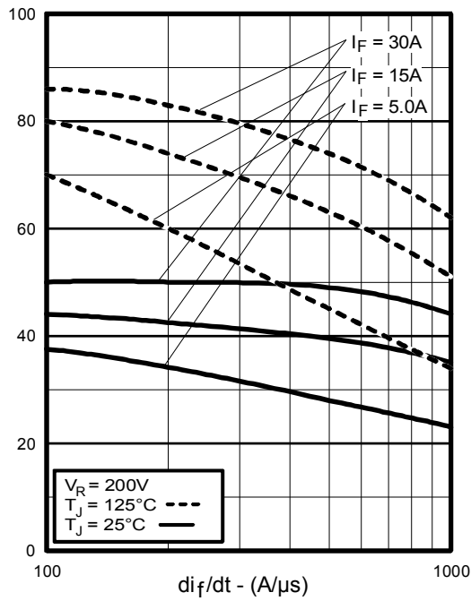
Fig. 5 - Typical Reverse Recovery vs. di/dt
