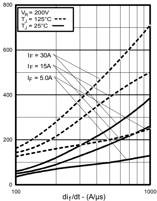
Fig. 7 - Typical Stored Charge vs. di/dt
