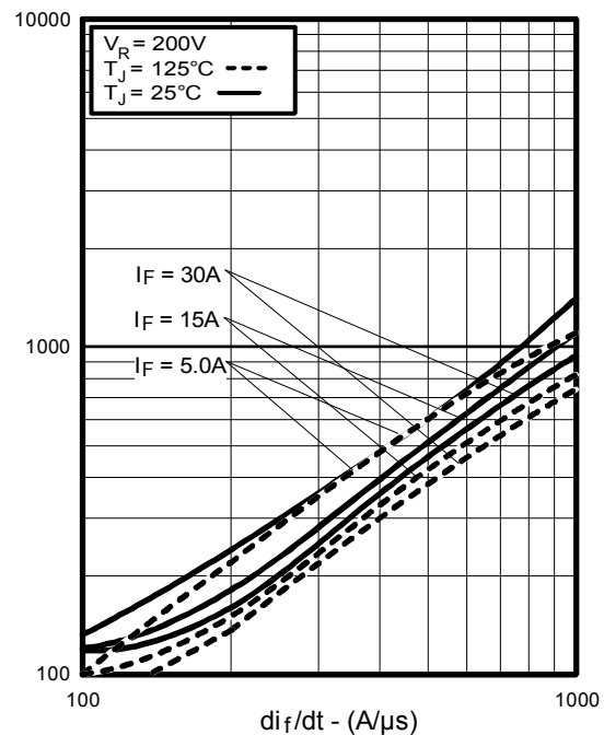
Fig. 8 - Typical di_{(rec)}M/dt vs. di/dt
