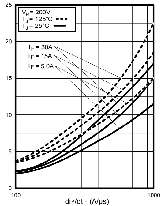
Fig. 6 - Typical Recovery Current vs. di/dt
