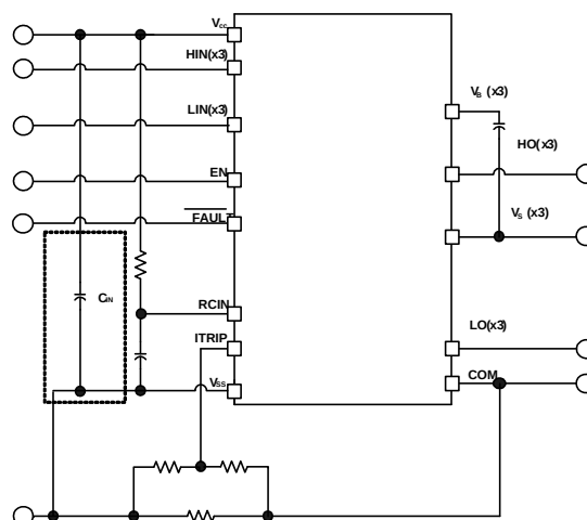
Figure 35: Supply capacitor
