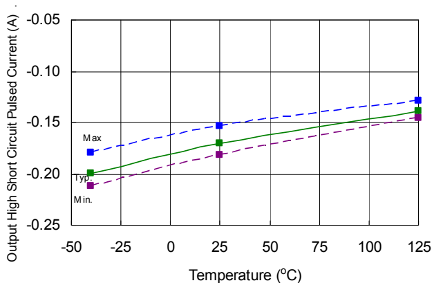
Figure 50: I_{O+} vs. temperature
