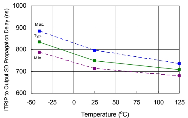
Figure 41: t_{TRIP} vs. temperature
