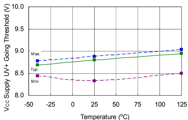
Figure 52: V_{CCUV+} vs. temperature
