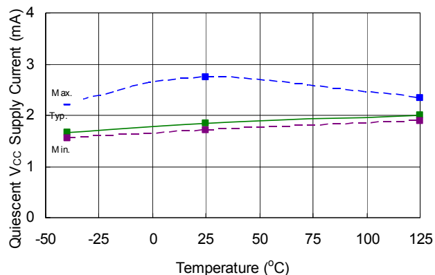
Figure 48: I_{QCC} vs. temperature
