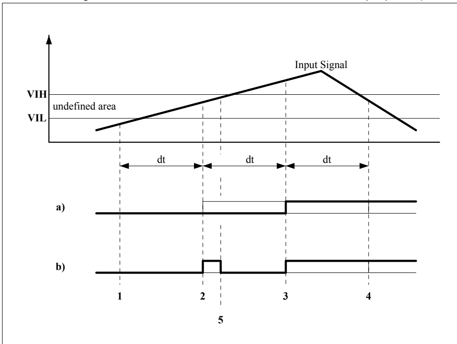
Figure 1 Input Signal Rise and Fall Times
