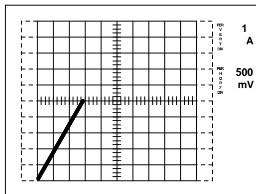
Figure 8. Drain-source resistance
