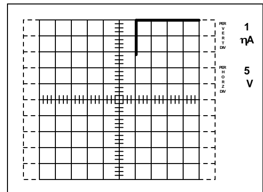
Figure 6. Gate-source leakage current at -20 V
