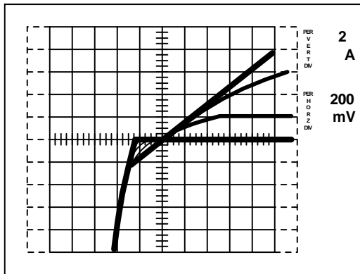
Figure 10. Operation in first and third quadrant (synchronous rectification)
