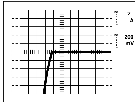
Figure 11. Operation in first and third quadrant without gate drive
