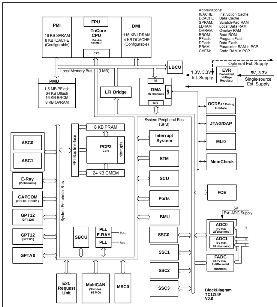
Figure 1 SAK-TC1724F-192F133HL / SAK-TC1724F-192F133HR Block Diagram
