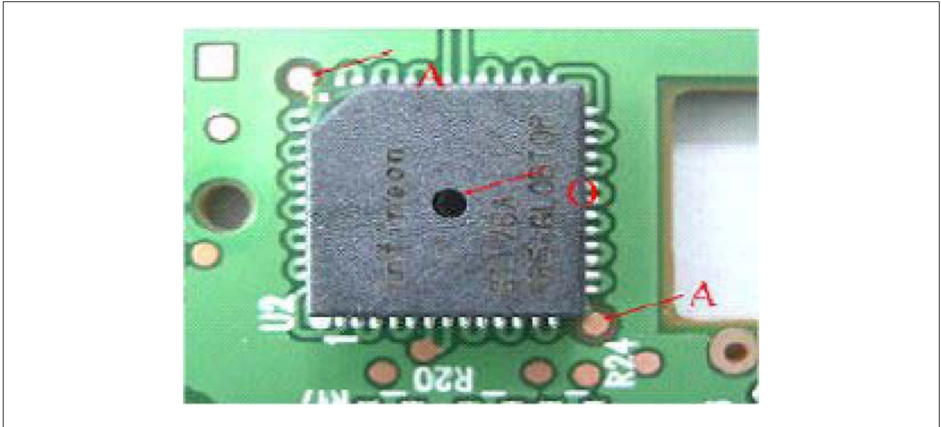
Figure 7 Overview on a Soldered PG-OCCN Package
