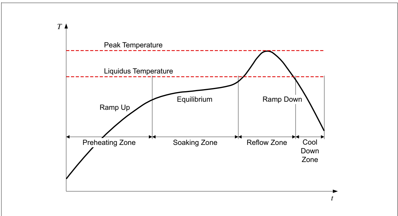
Figure 5 General Forced Convection Reflow Solder Profile
