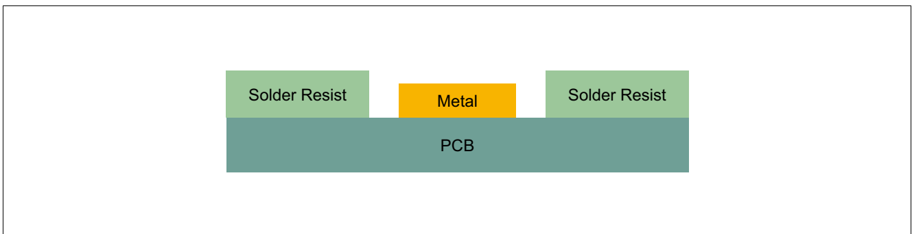
Figure 3 NSMD Pad
