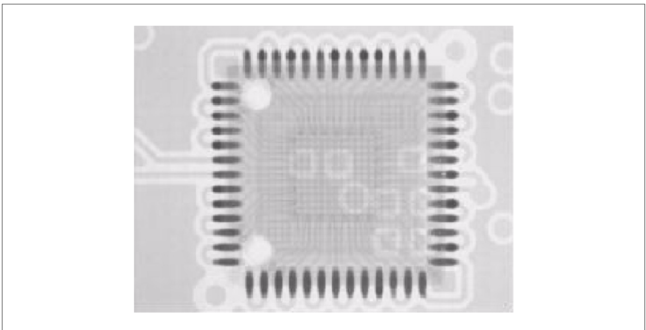
Figure 8 Typical X-ray Image of Soldered PG-OCCN Package
