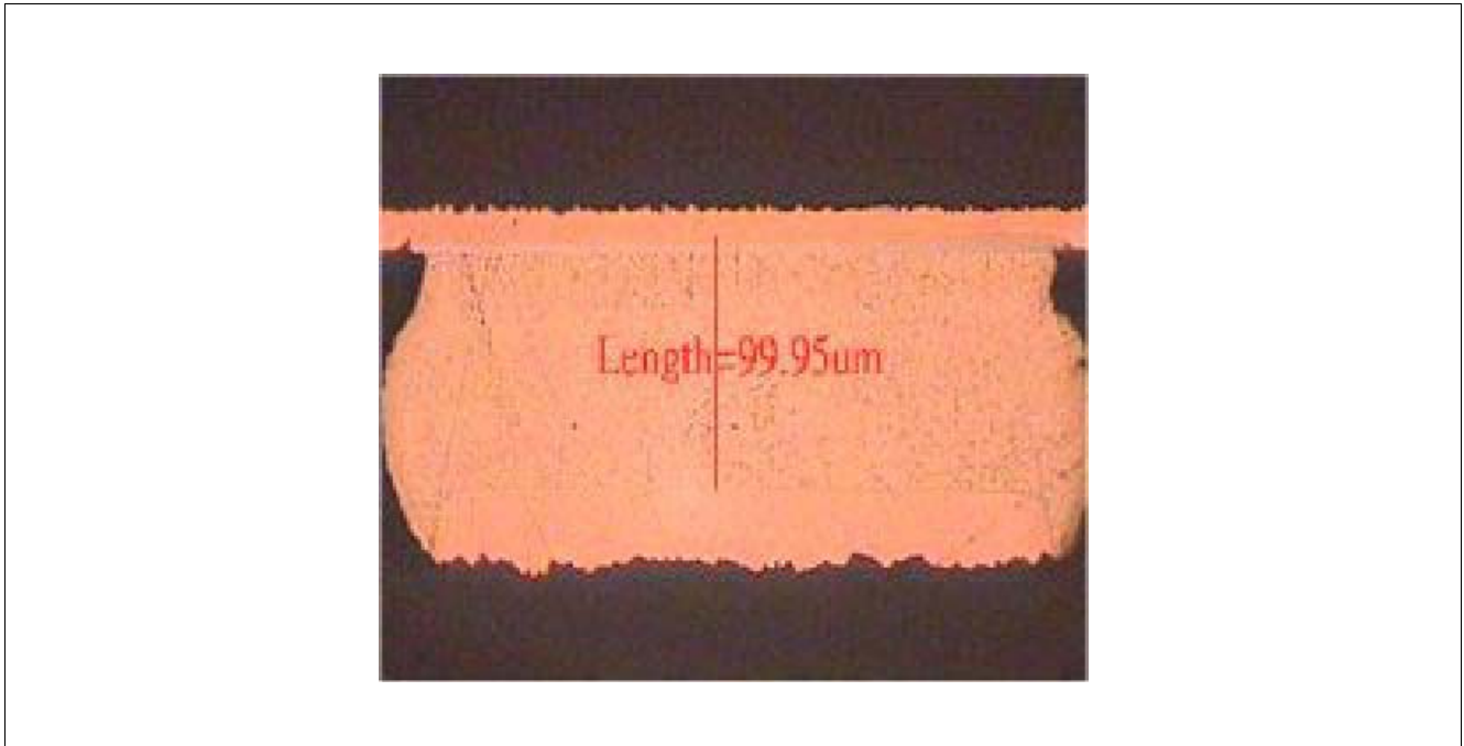
Figure 9 Cross Section of a PG-OCCN Solder Joint
