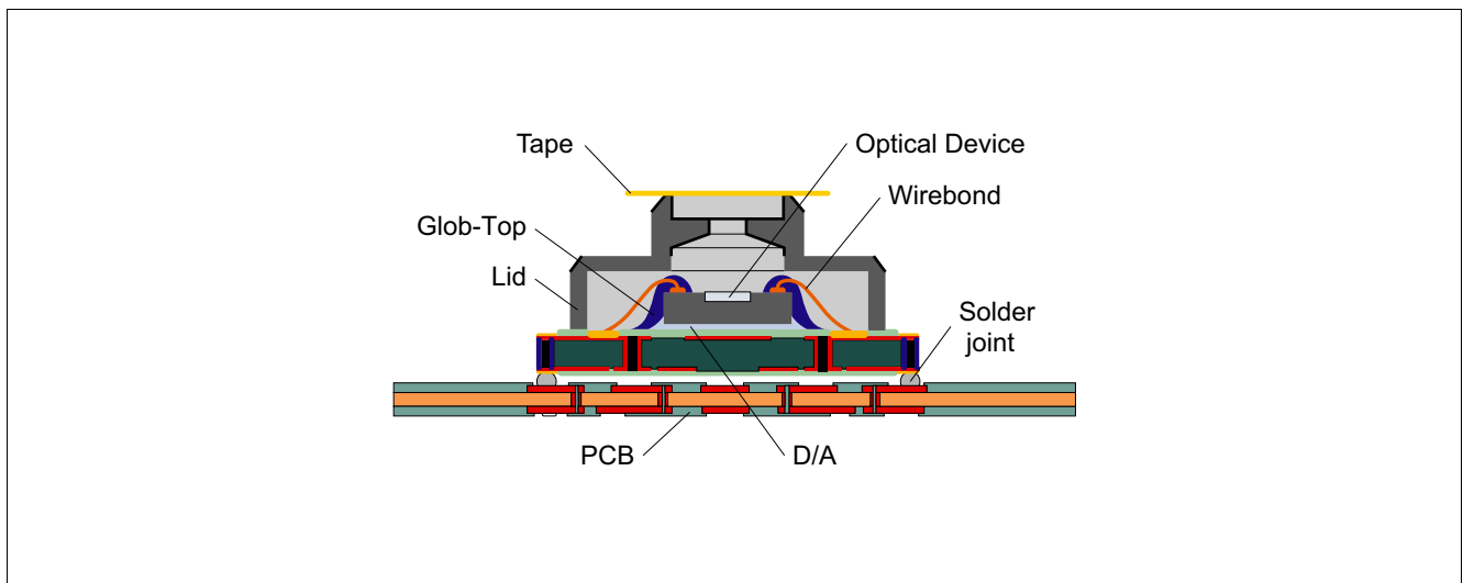
Figure 1 PG-OCCN Cross Section (mounted on PCB)
