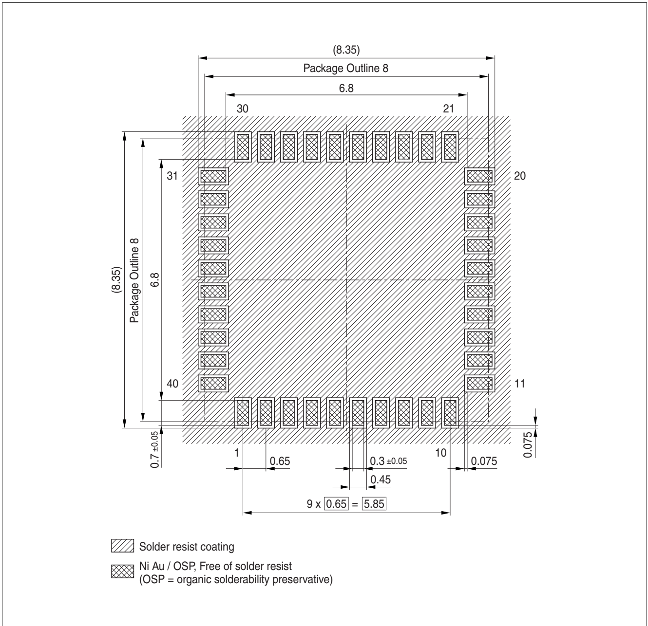
Figure 4 PCB Pad Design Recommendation
