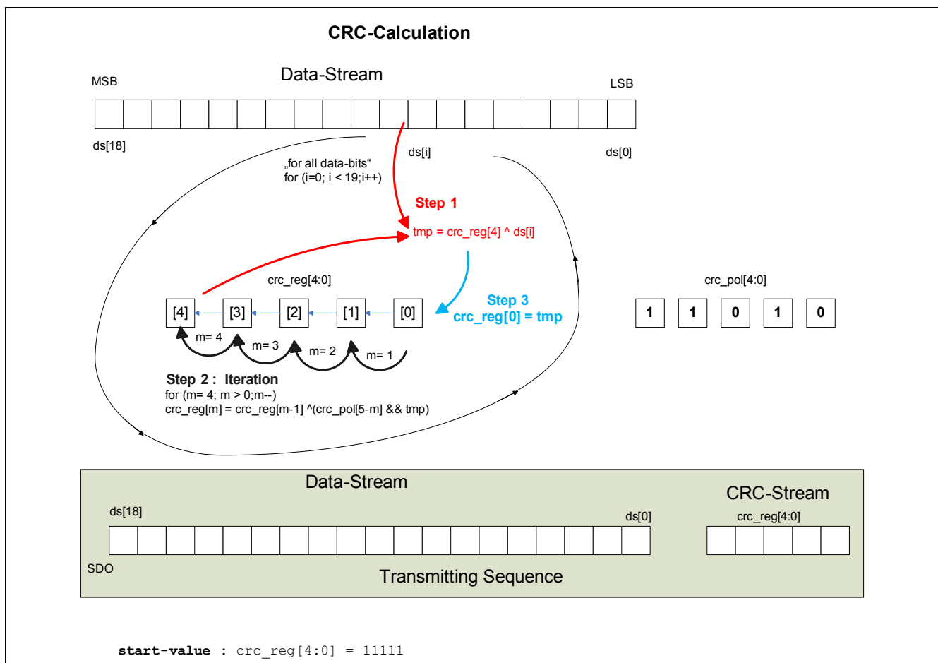
Figure 28 CRC-Calculation
