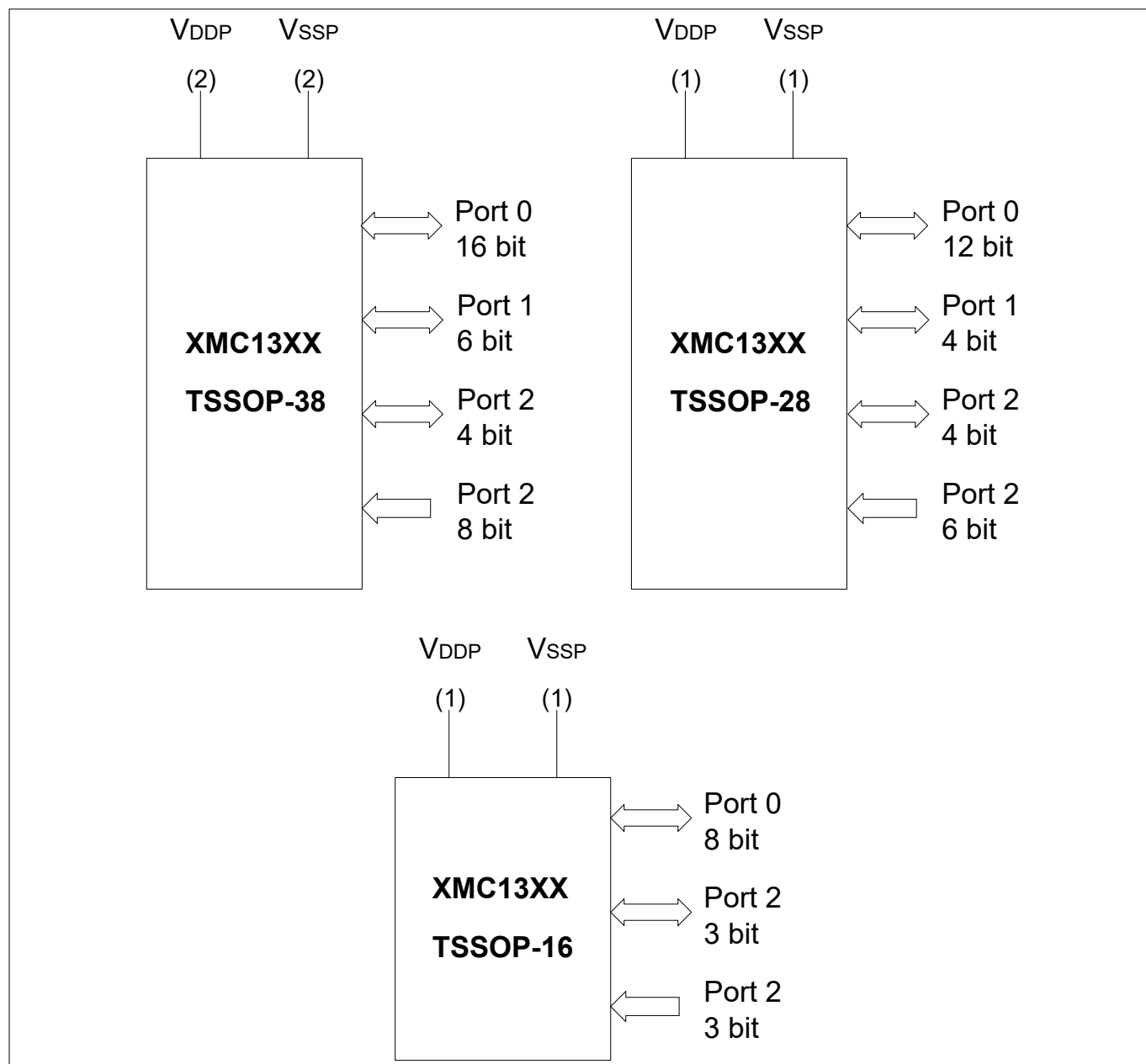
Figure 2 XMC1300 Logic Symbol for TSSOP-38, TSSOP-28 and TSSOP-16
