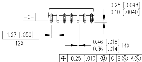
14 Lead SOIC (narrow body)
