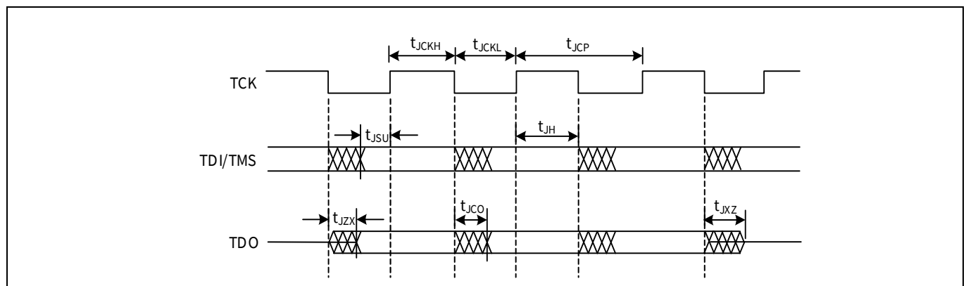
Figure 30 JTAG specifications
