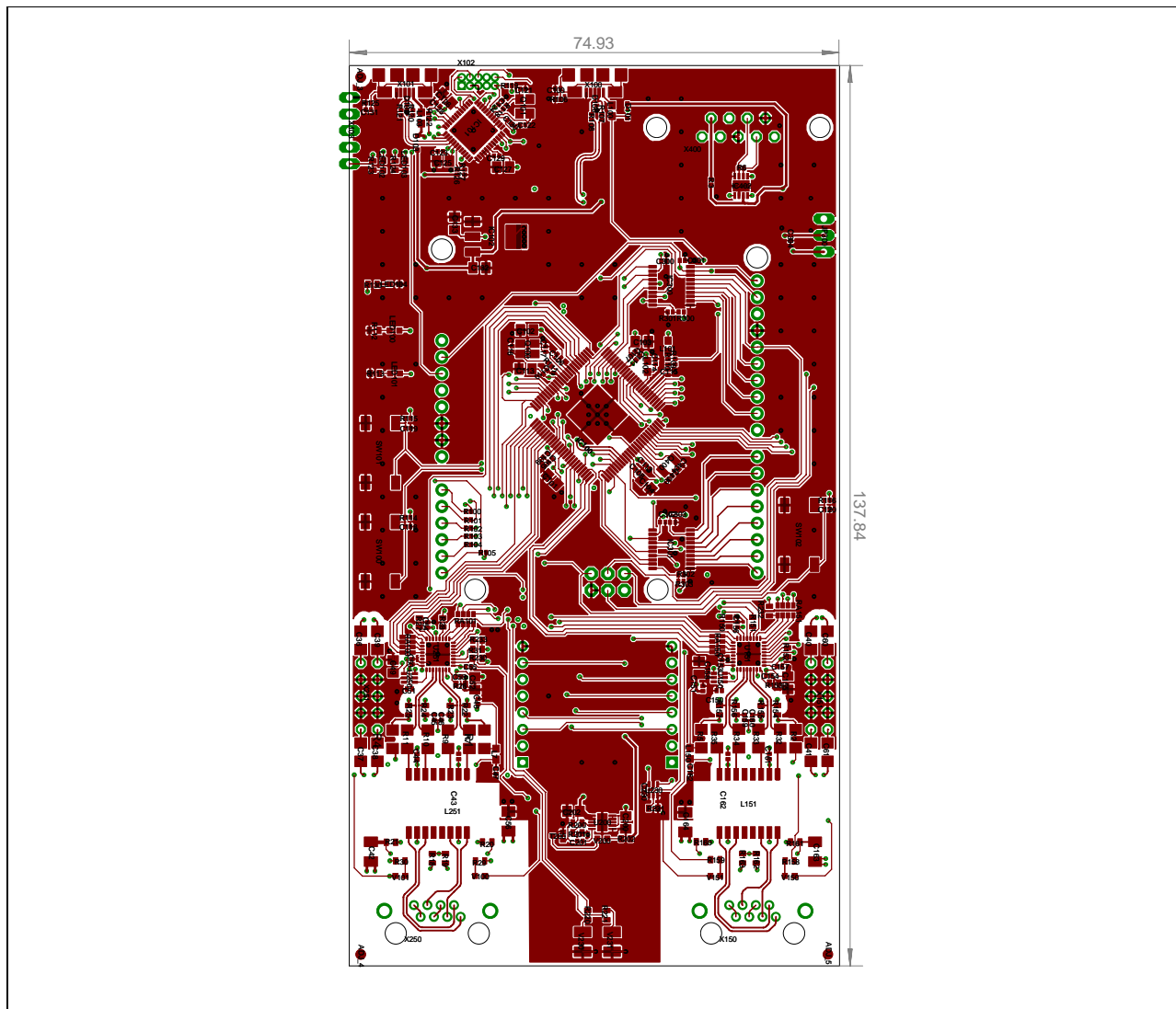
Figure 11 Components placement and geometry
