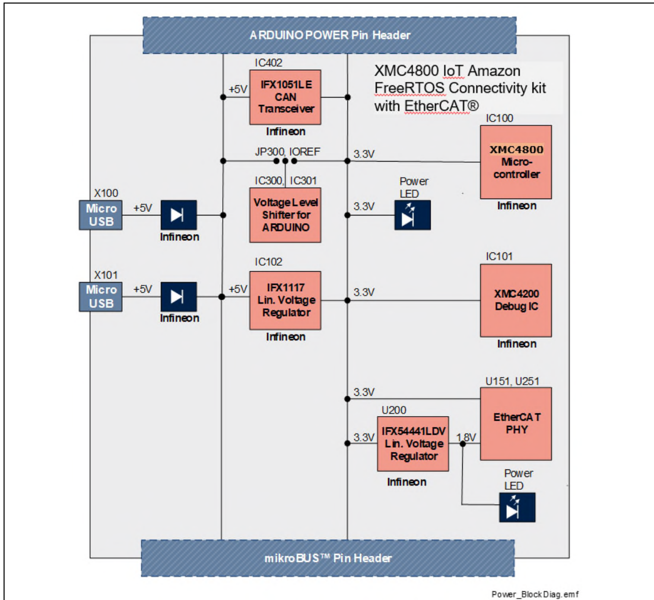
Figure 3 Power supply concept
