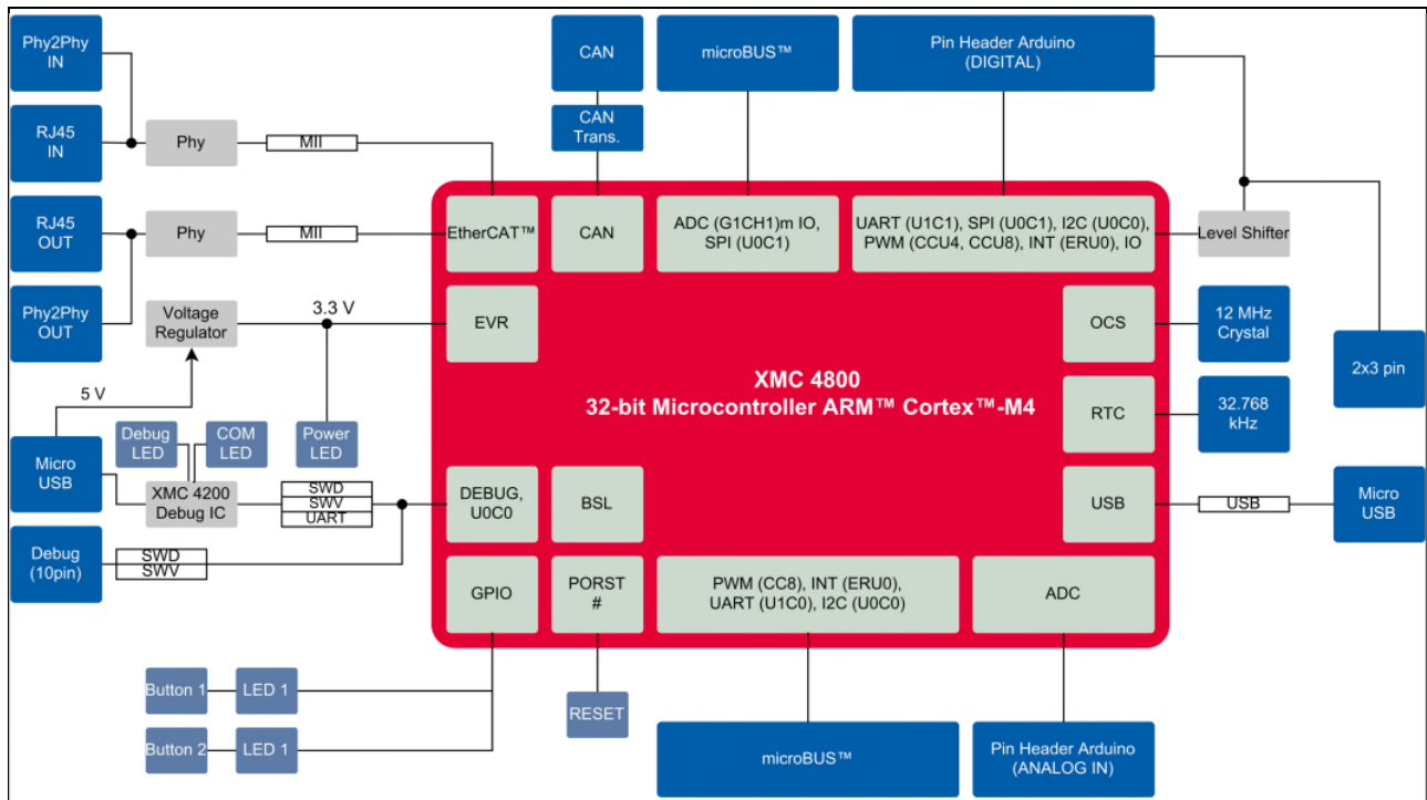
Figure 1 Block diagram of the XMC4800 IoT Amazon FreeRTOS Connectivity kit with EtherCAT®
