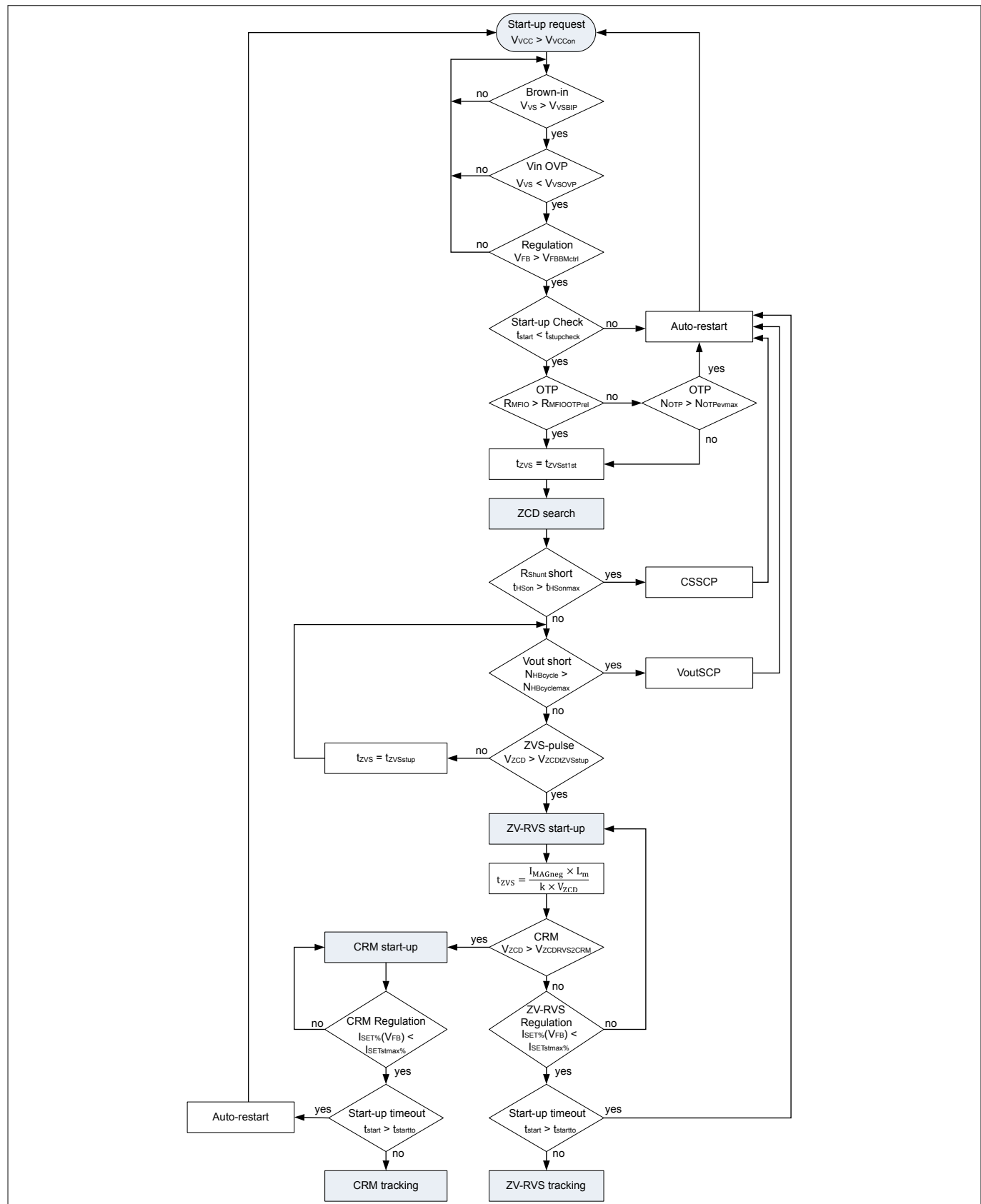
Figure 34 Start-up sequence
