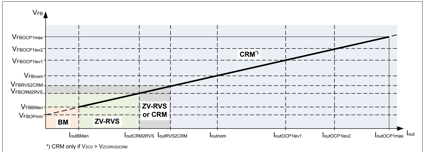
Figure 24 Control law for feedback voltage at FB pin
