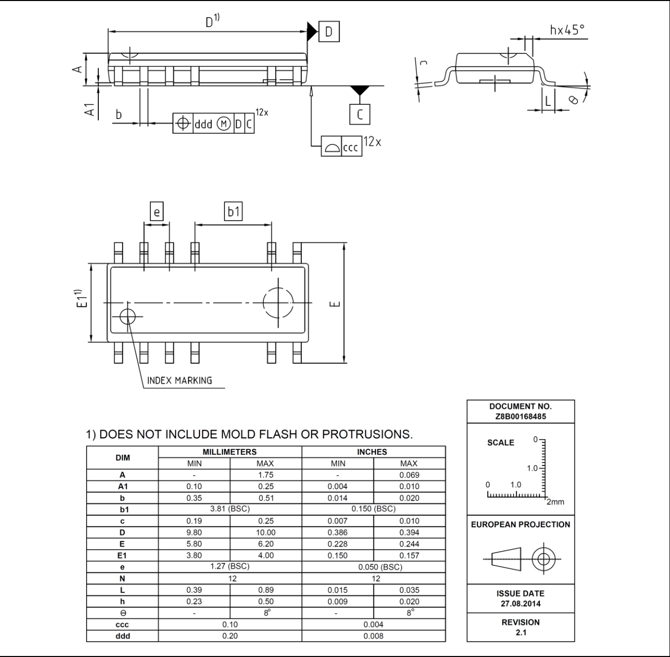
Figure 31 PG-DSO-12 Package Outline
