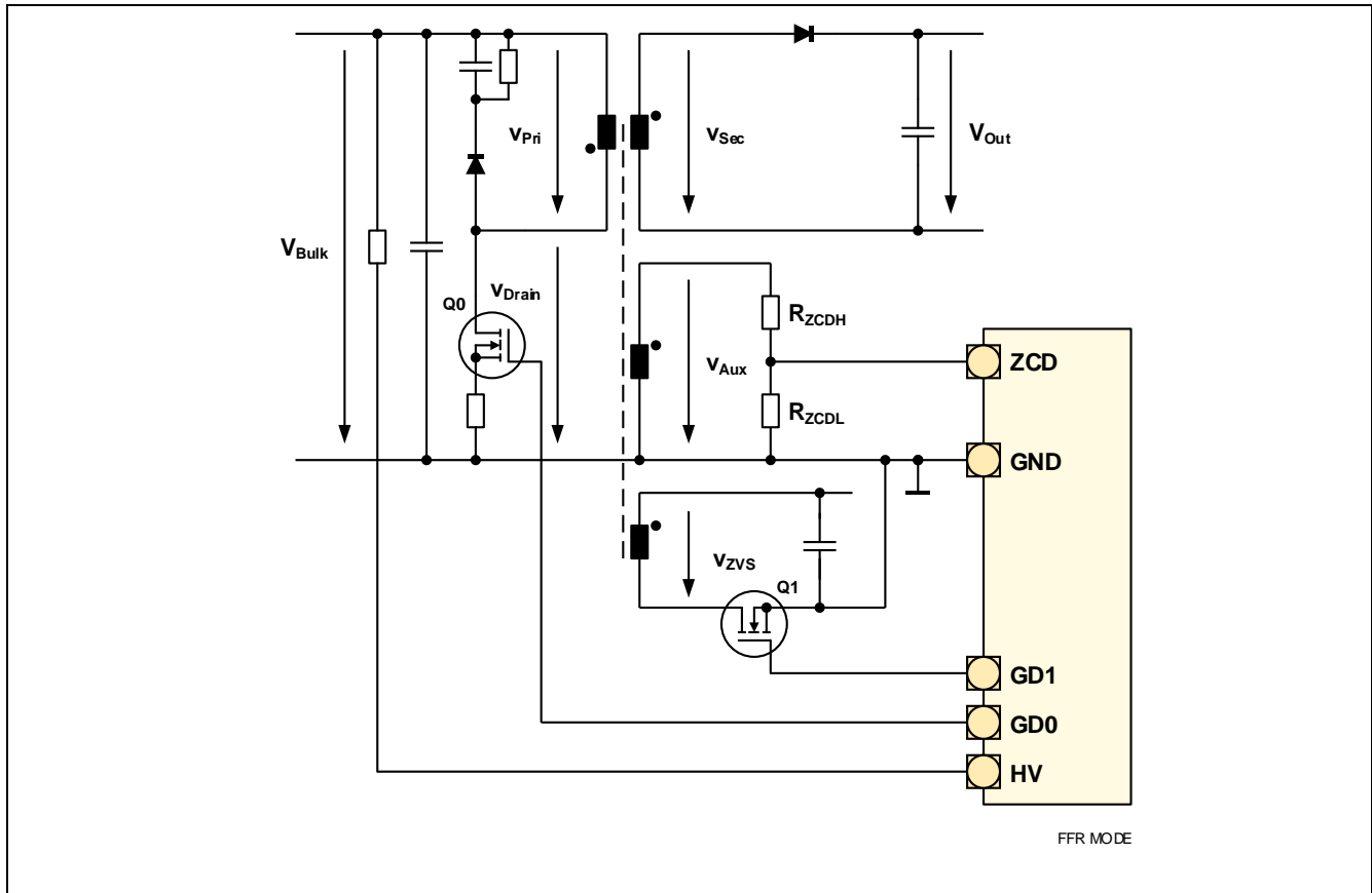
Figure 28 Required signals for forced quasi resonant ZVS mode operation
