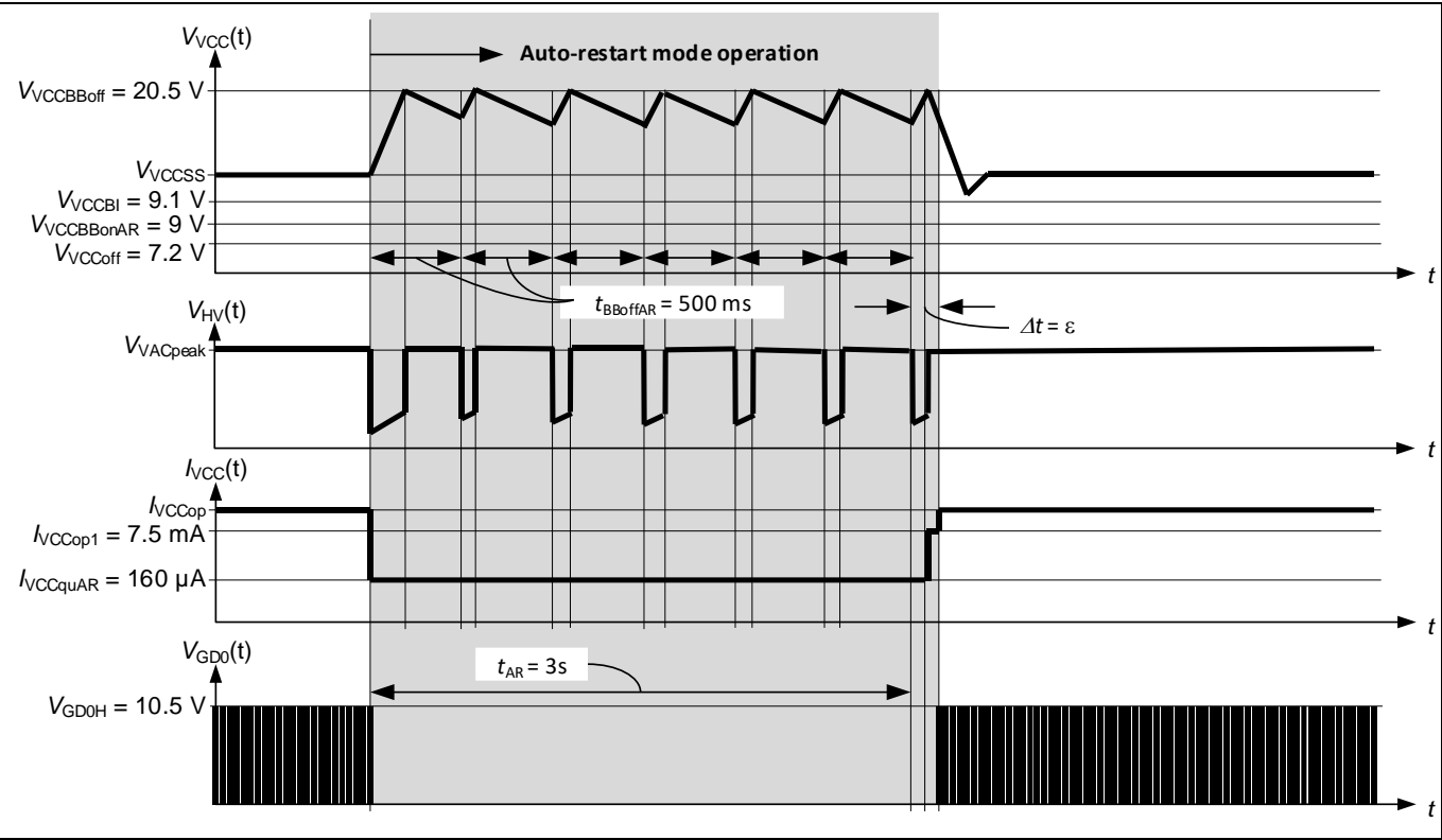
Figure 10 Auto-restart mode operation
