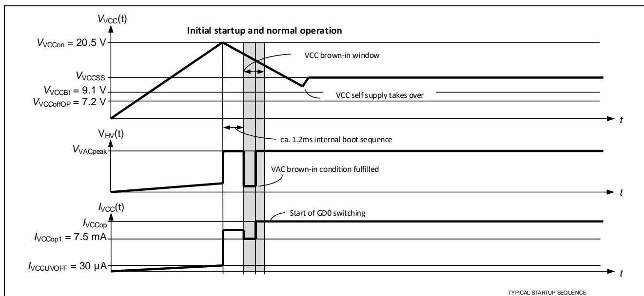
Figure 4 Typical startup sequence
