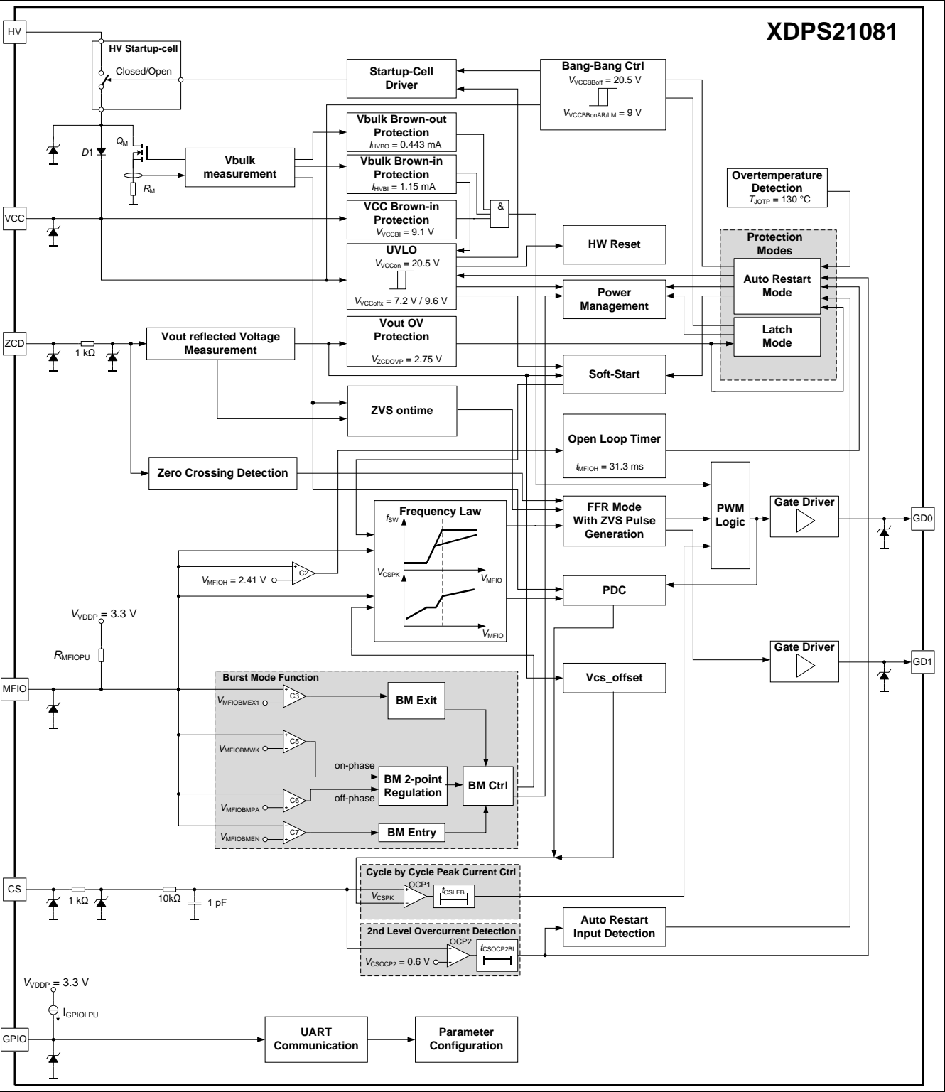
Figure 3 Representative Block Diagram of XDP21081
