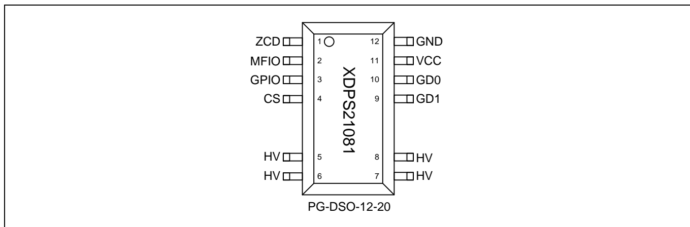
Figure 2 Pin Configuration of XDP21081
