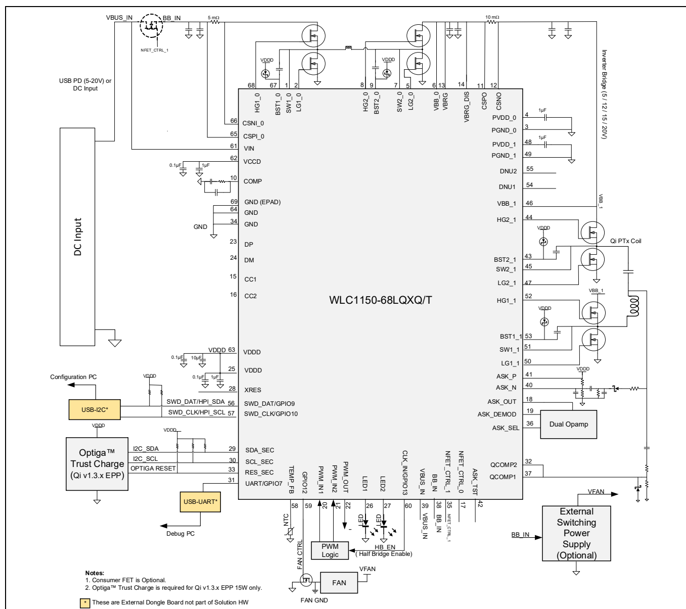
Figure 2 Application diagram for dual stage 50W transmitter solution with integrated buck-boost controller
