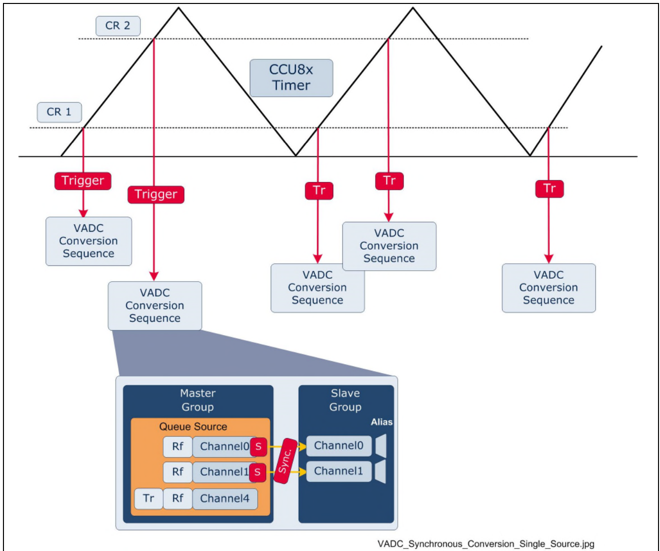
Figure 15 Single Source Synchronization Example
