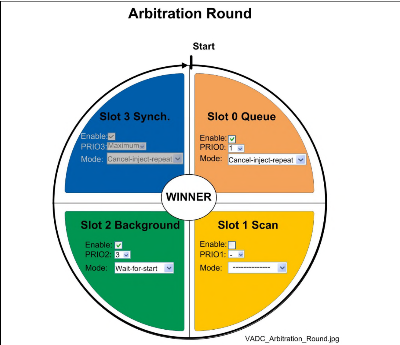
Figure 29 Arbitration schema
