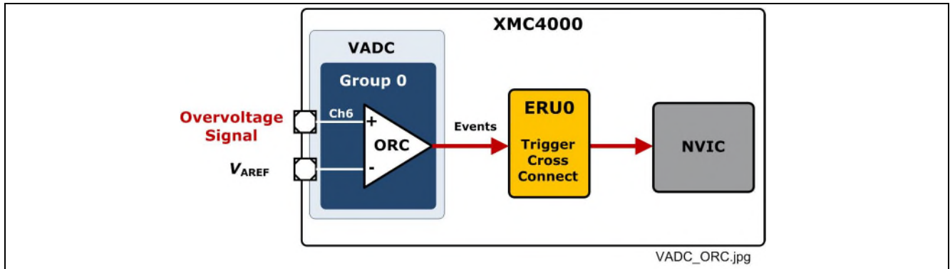
Figure 70 Out of Range Comparator
