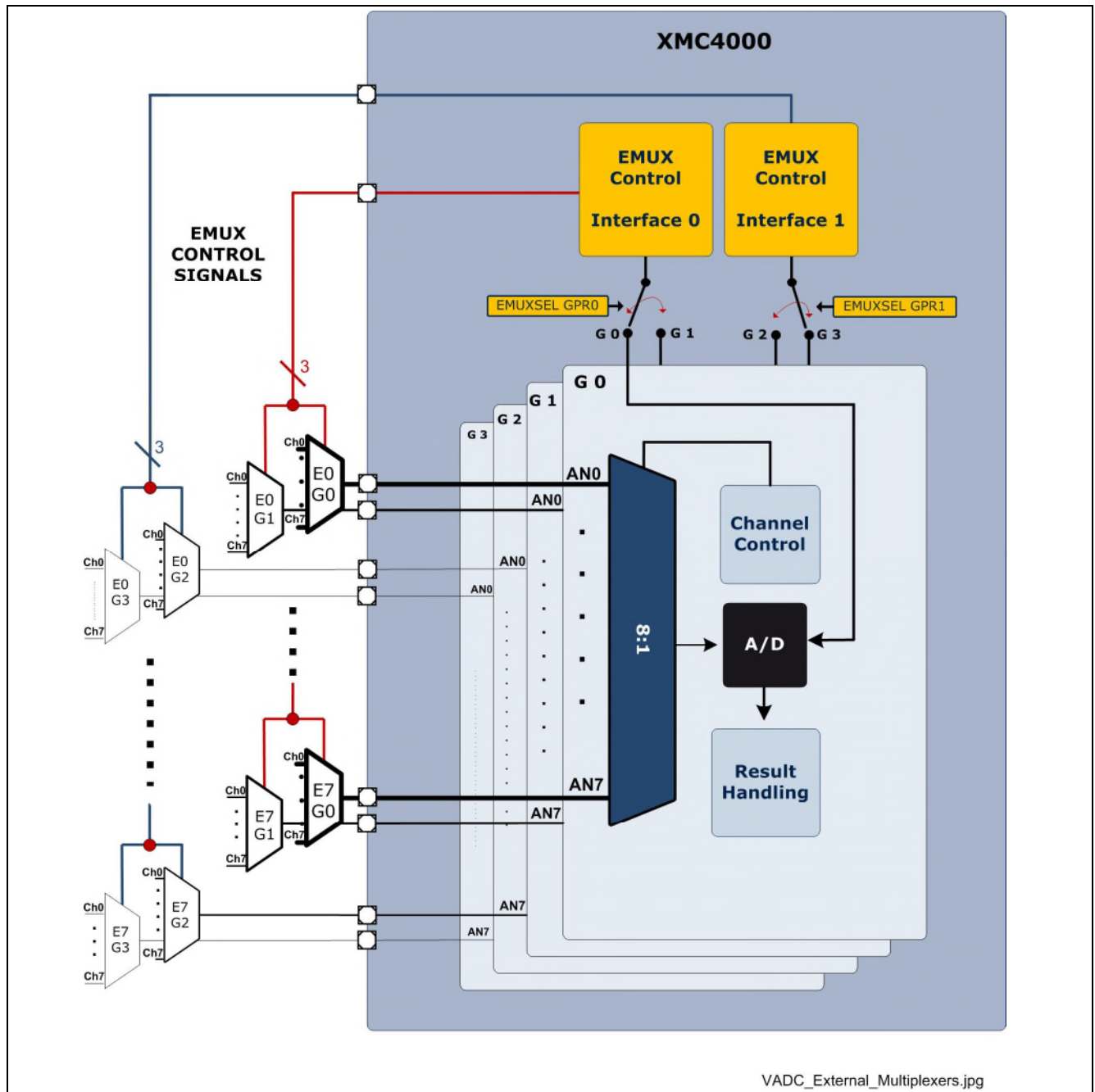
Figure 73 External Multiplexers
