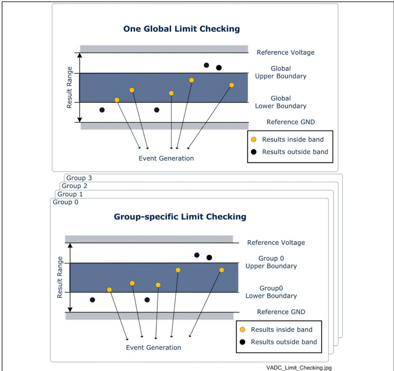
Figure 63 Global and Group-specific Limit Checking
