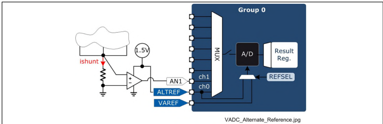
Figure 26 Selecting the Alternate Reference on ch0 via REFSEL
