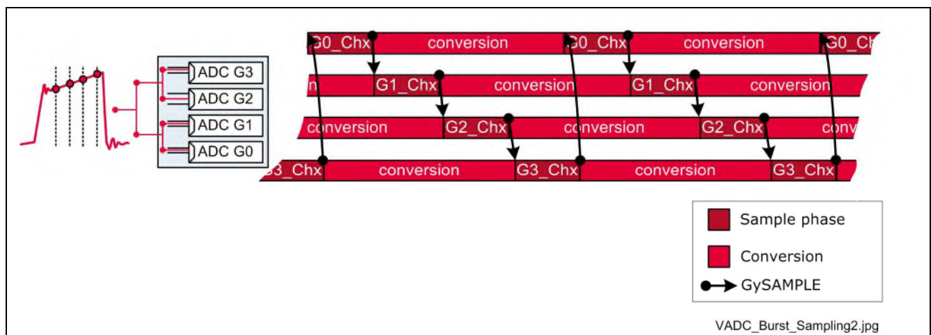
Figure 48 Burst sampling
