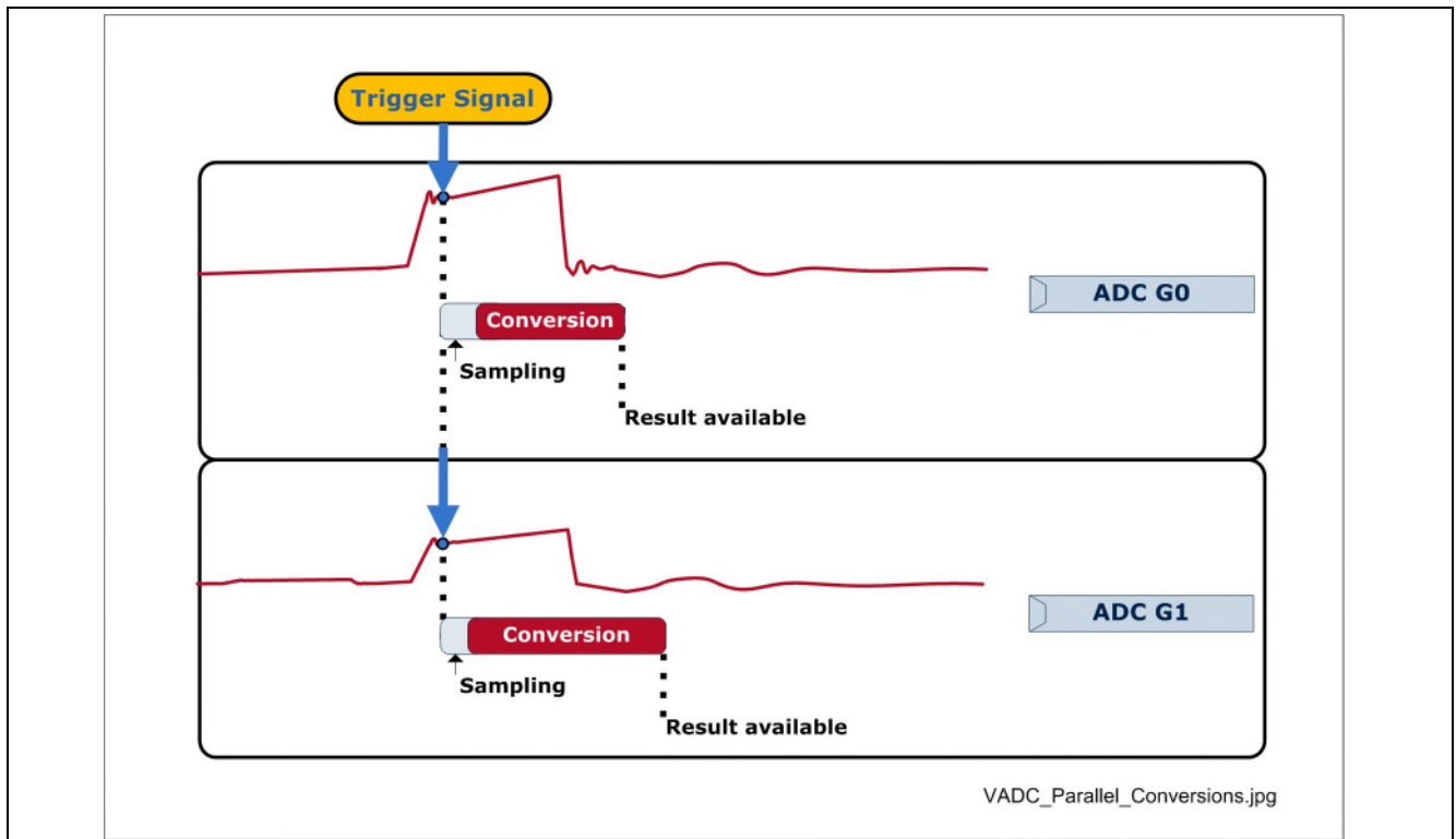
Figure 12 Parallel conversions
