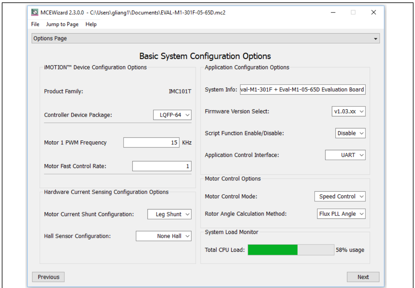
Figure 12 Shunt configuration
