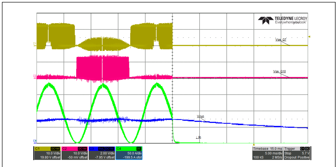
Figure 53 Over-load shut-down showing I_{run} input to U2 V_{gs\_Q7} (yellow), I_{pri} (red), V_{run} (blue), V_{pri} (green)
