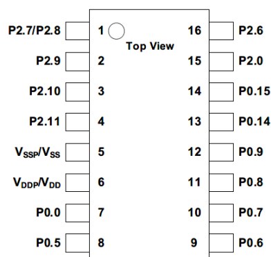
Figure 19 XMC1300 PG-TSSOP-16 pin configuration (top view)
