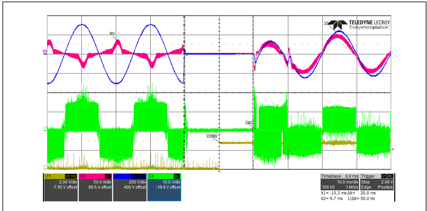
Figure 48 Switching to back-up mode when AC power fails at 263 W resistive load V_{\text{relay}} (yellow), V_{\text{OUT}} (blue), I_{\text{pri}} (red), V_{\text{pri}} (green)
