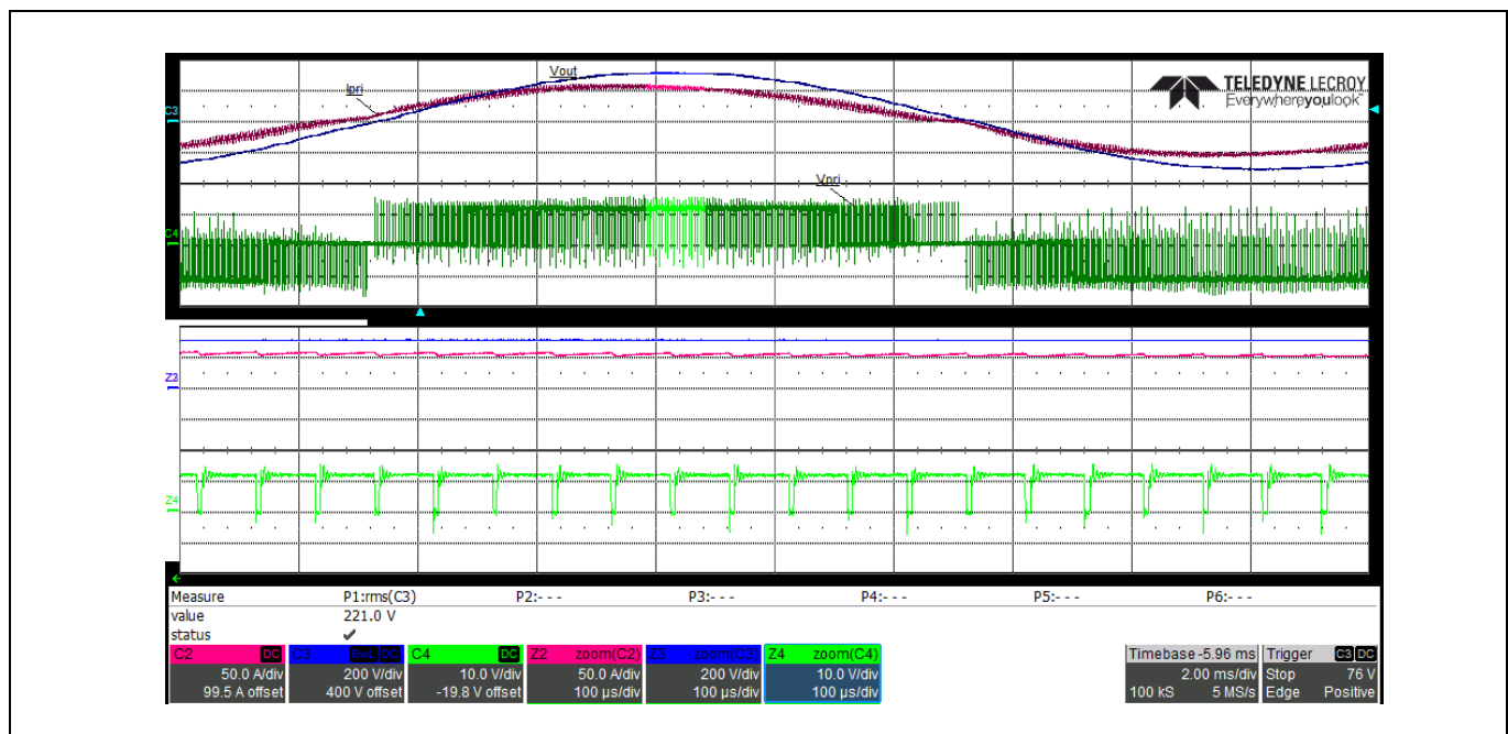
Figure 47 Primary voltage waveform at 263 W resistive load
