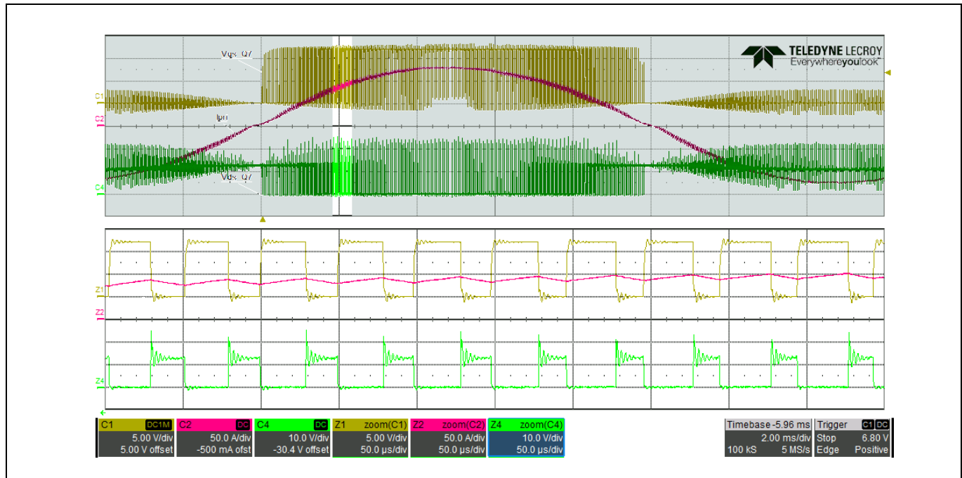
Figure 46 Primary current waveform at 672 W resistive load
