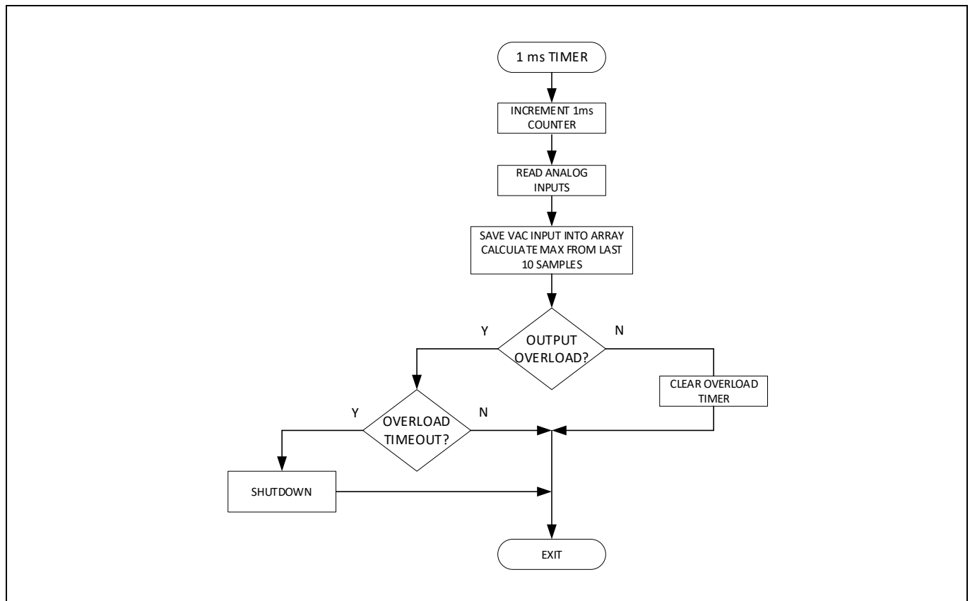
Figure 29 1 ms routine
