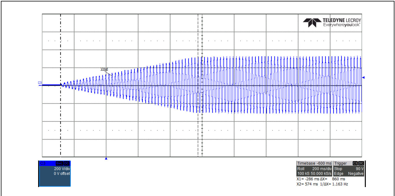
Figure 38 Start-up at zero load Output voltage (blue)
