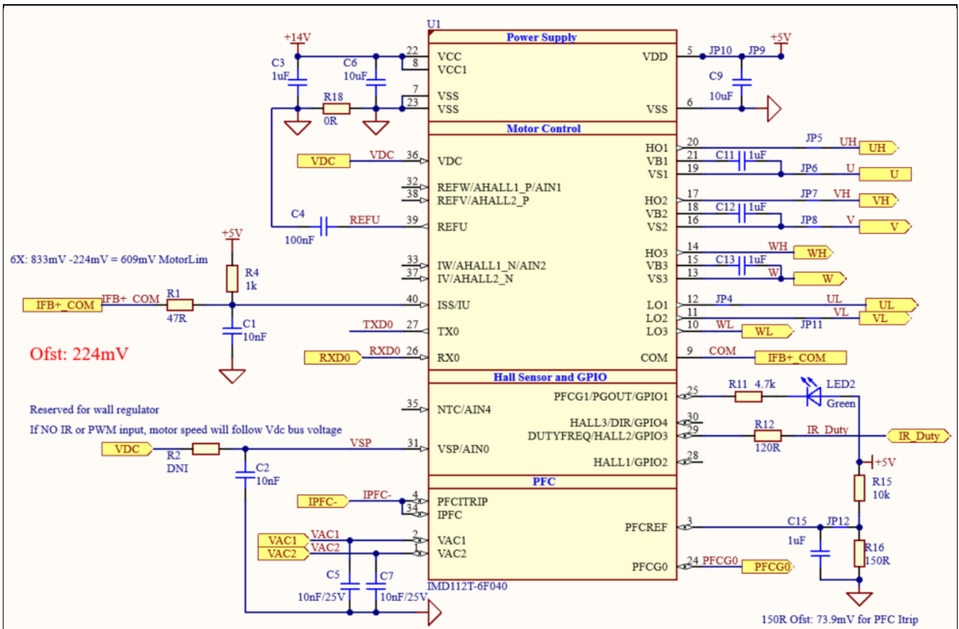
Figure 32 Interface circuit of IMD112T
