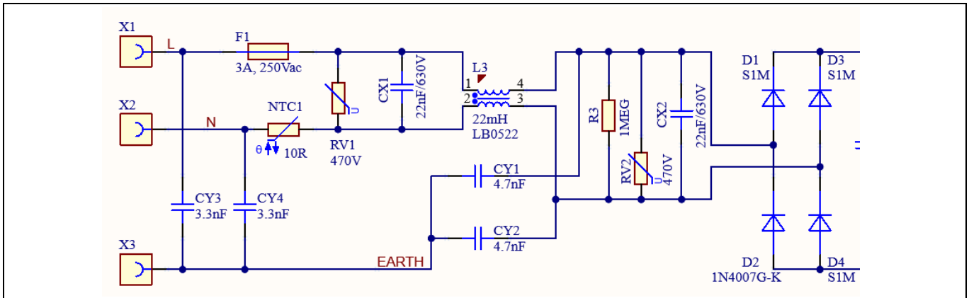
Figure 21 EMI filter and surge protection
