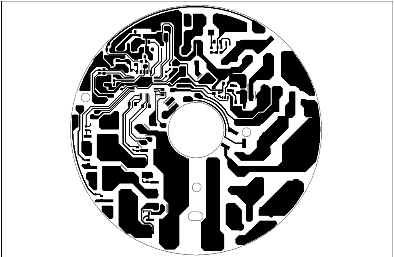
Figure 40 Bottom layer of the main board
