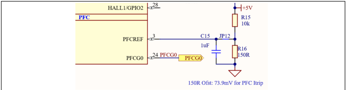
Figure 31 PFC overcurrent threshold design on the board
