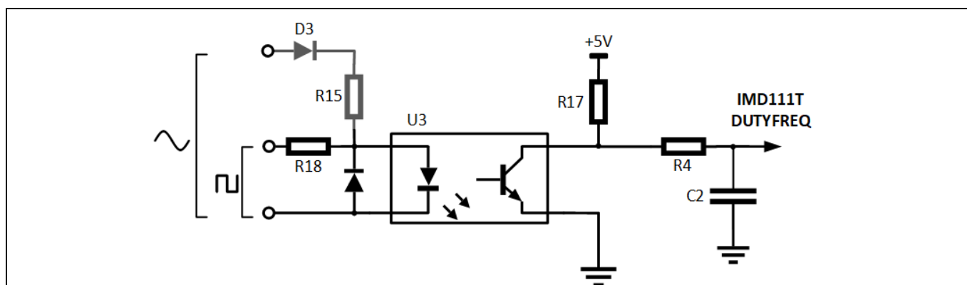
Figure 18 Frequency-interface circuit
